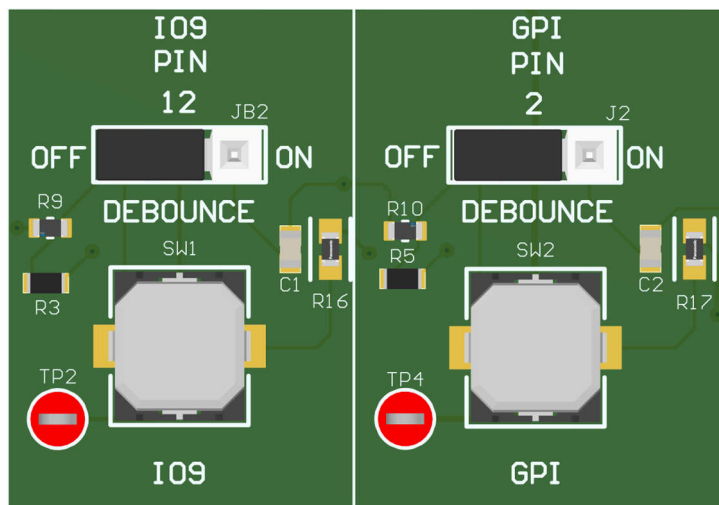
Figure 2-4. Switch Blocks
