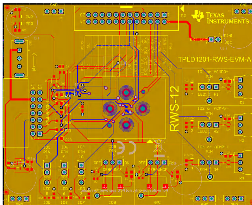
Figure 4-2. TPLD1201-RWS-EVM Layout
