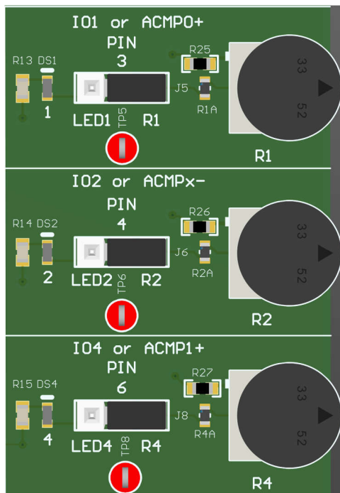
Figure 2-5. LED/POT Blocks
