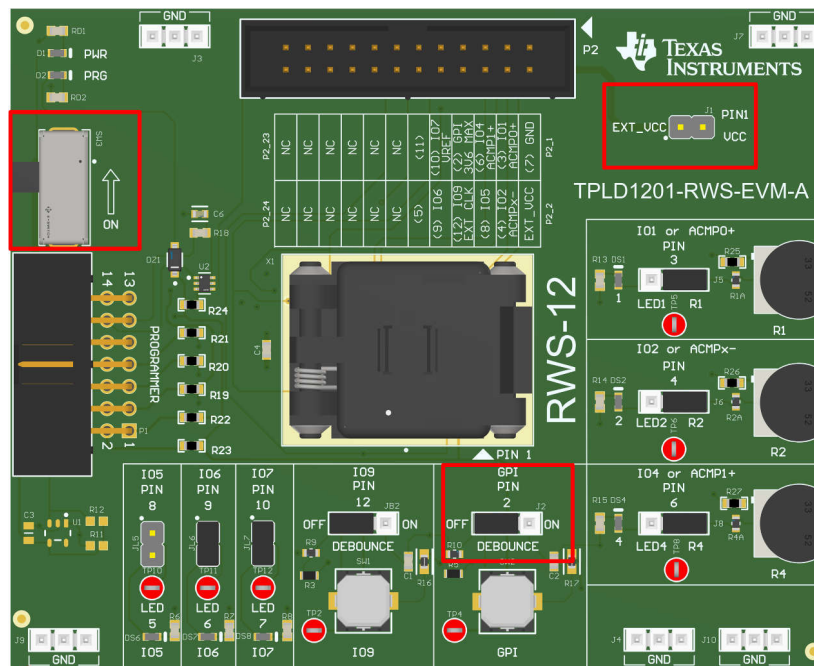
Figure 3-2. Components Considered in Programming Setup
