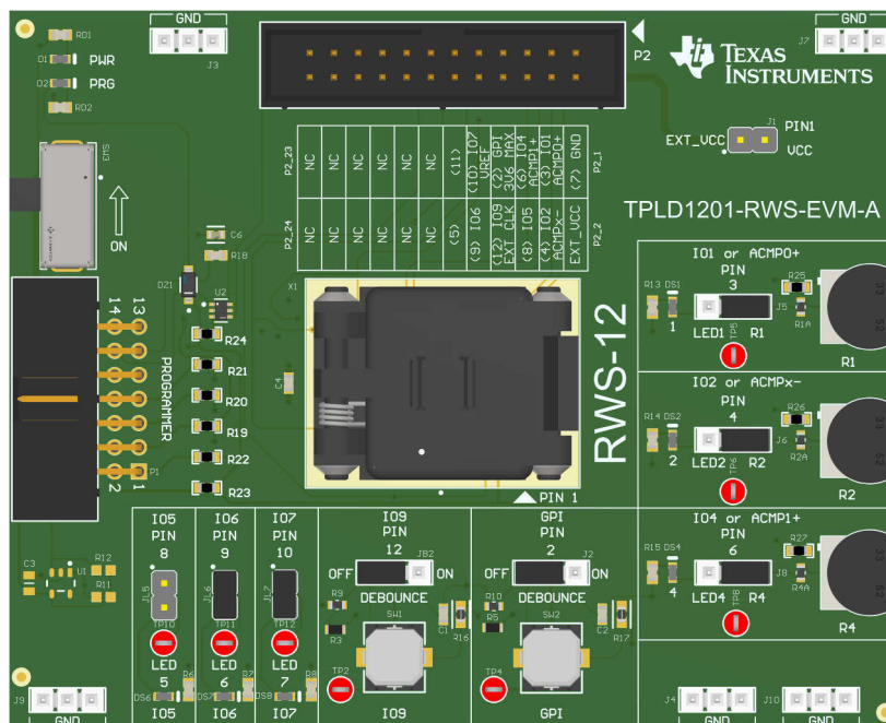
Figure 4-3. TPLD1201-RWS-EVM Board Front
