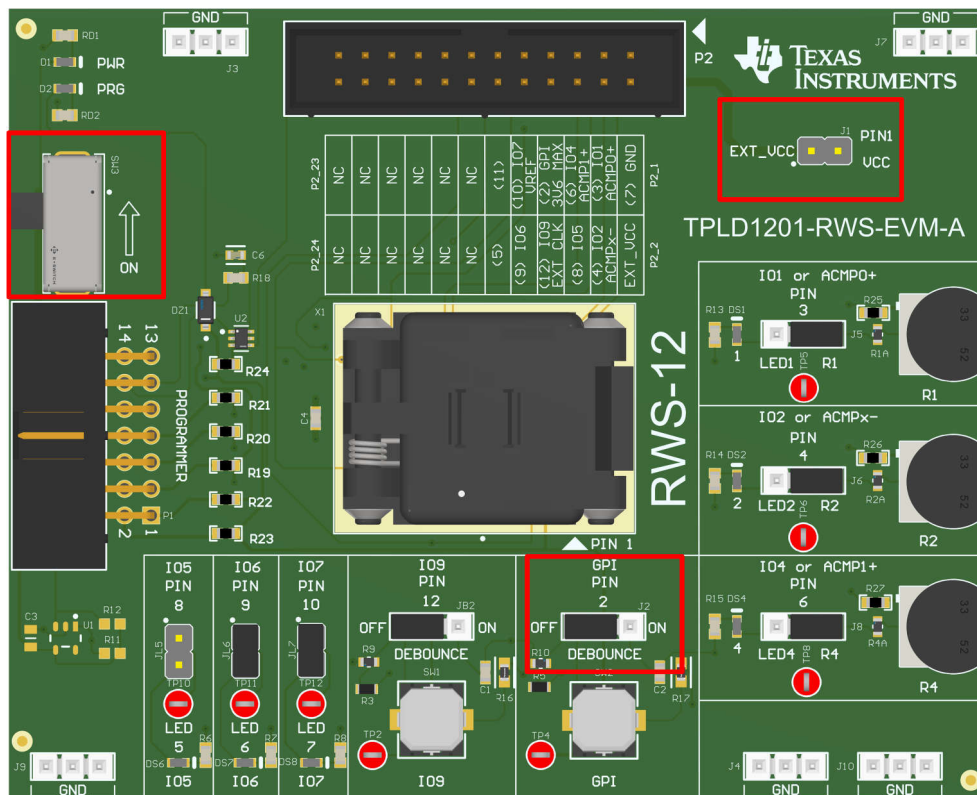
Figure 3-9. Headers and Switches used in Demo Configuration
