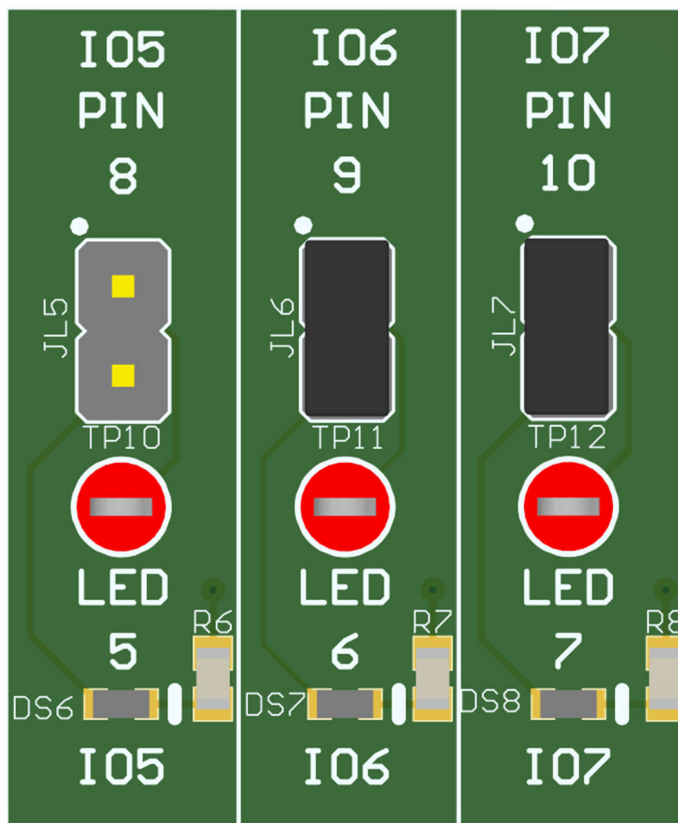
Figure 2-3. LED Blocks
