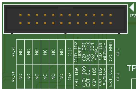
Figure 2-1. P2 and J1 Headers
