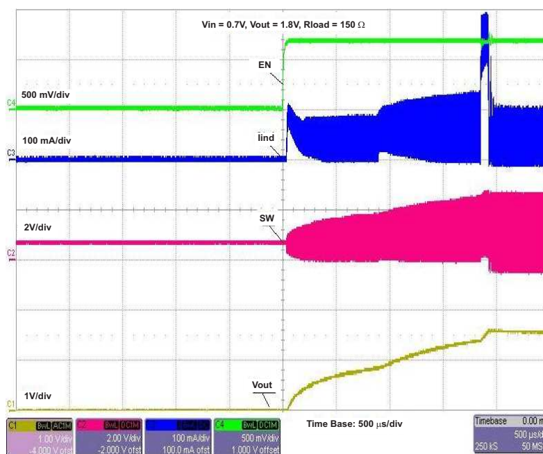
Figure 3. Start-Up After Enable
