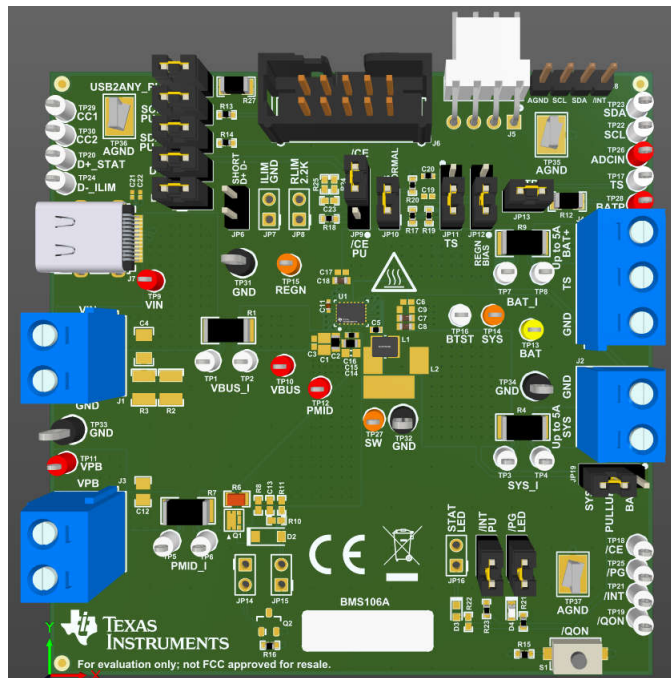
BQ25640EVM Hardware Board
