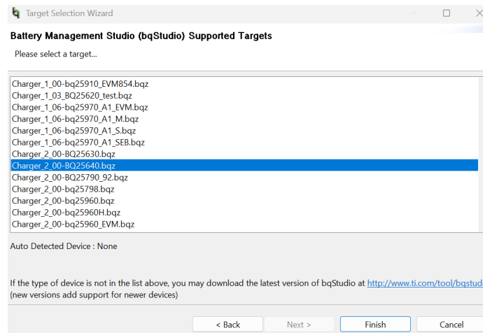
Figure 3-2. BQStudio Charger Selection Window (choose Charger_2_00-bq25640.bqz)
