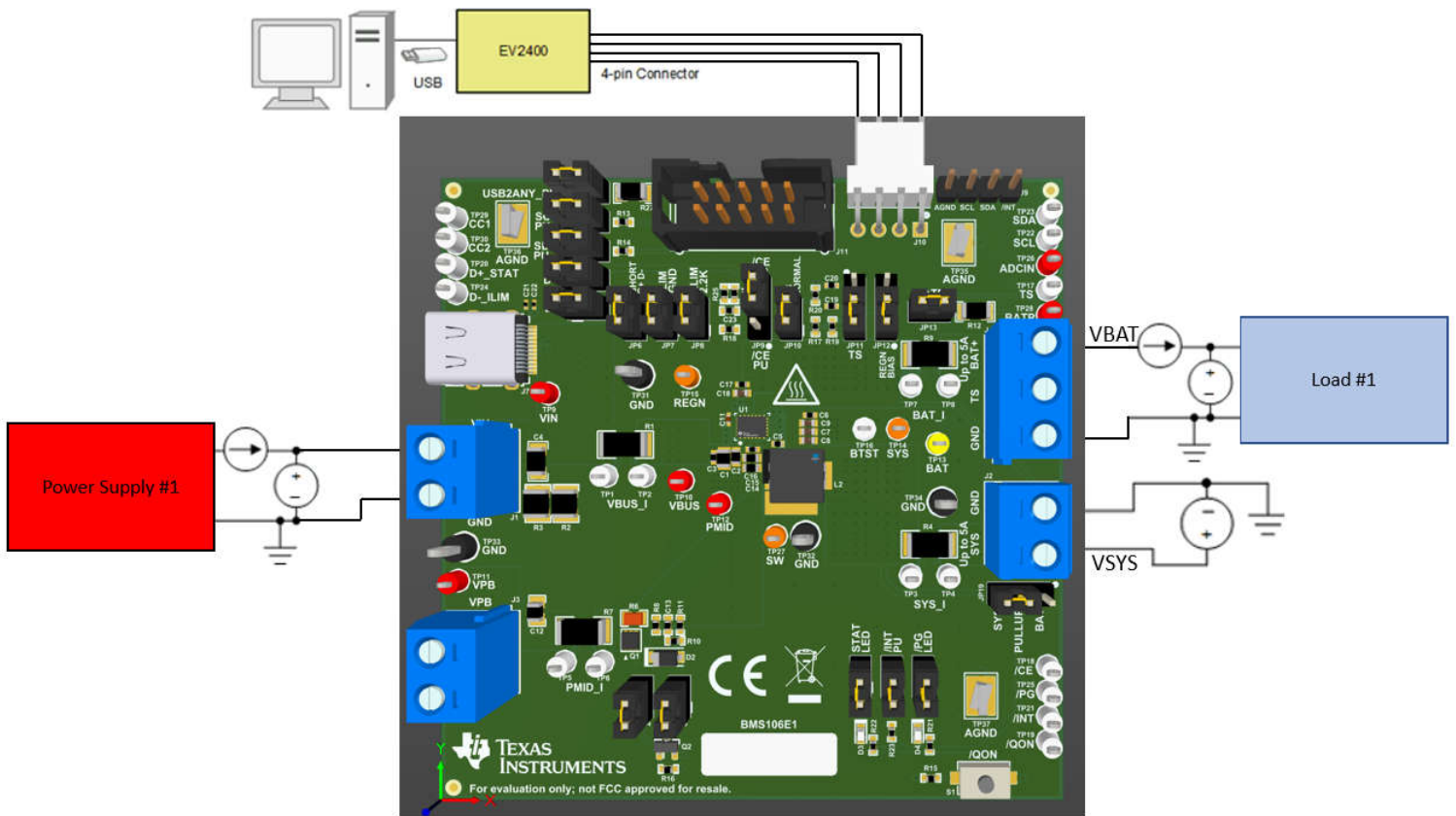
Figure 2-1. Test Setup for BQ25640 EVM
