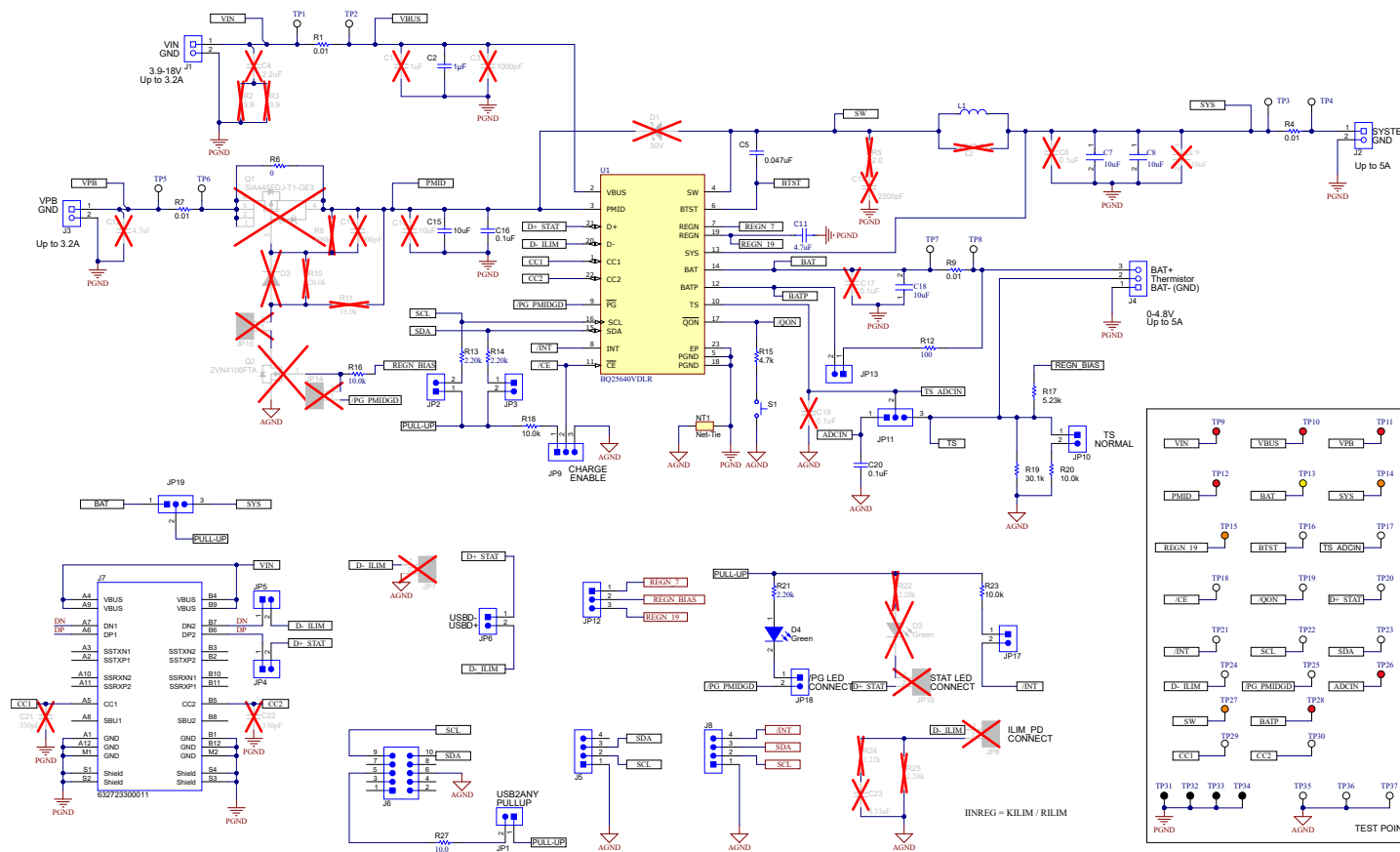
Figure 4-1. BQ25640EVM Schematic
