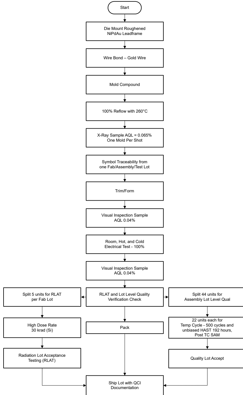
Figure 2-1. SN54SC6T06-SEP Space Enhanced Plastic Production Flow Chart
