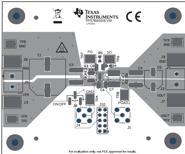
Figure 2. Assembly Layer
