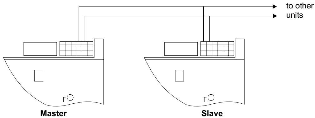
Figure 4-6. Carrier Phase Synchronisation Interface Connection
