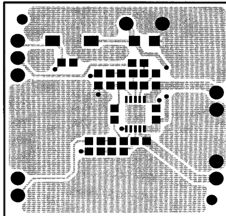
Figure 2–7. TPA6112A2 EVM Top Layer
