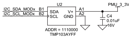
Figure 12. SMP-TPS61201-MVK Schematic
