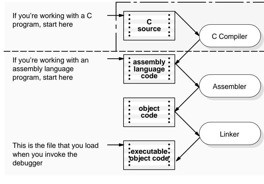
Figure 1–4. Steps You Go Through to Prepare a Program
