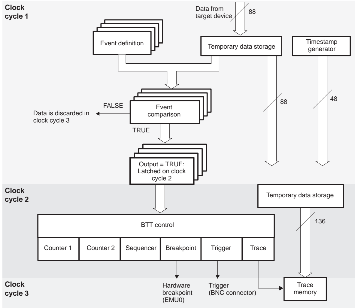
Figure 1–4. XDS522A Pipeline Architecture
