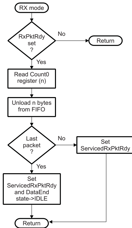
Figure 9. RX Mode Flow Chart
