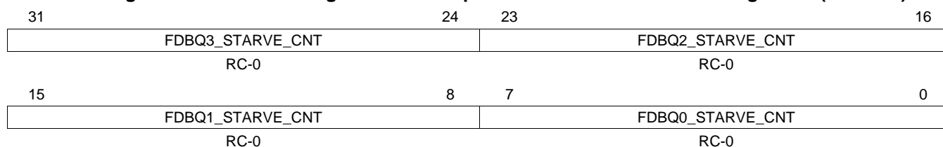
Figure 103. Queue Manager Free Descriptor/Buffer Starvation Count Register 0 (FDBSC0)
