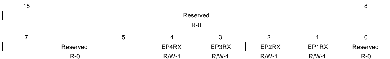
Figure 52. Interrupt Enable Register for INTRRX (INTRRXE)
