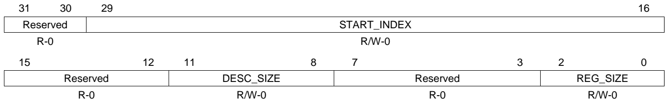
Figure 113. Queue Manager Memory Region R Control Registers (QMEMRCTRL[ R ])
