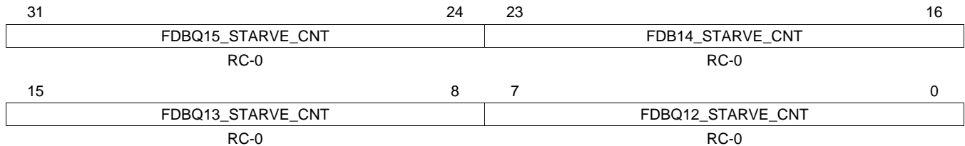
Figure 106. Queue Manager Free Descriptor/Buffer Starvation Count Register 3 (FDBSC3)
