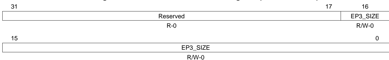
Figure 45. Generic RNDIS EP3 Size Register (GENRNDISSZ3)
