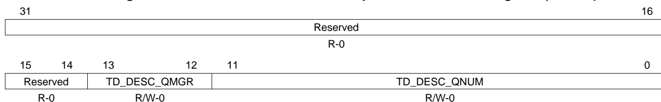
Figure 93. CDMA Teardown Free Descriptor Queue Control Register (TDFDQ)
