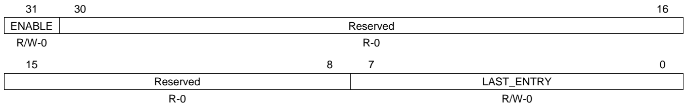
Figure 99. CDMA Scheduler Control Register (DMA_SCHED_CTRL)
