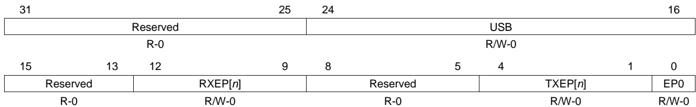
Figure 40. USB Interrupt Mask Clear Register (INTMSKCLRR)
