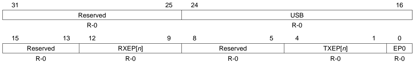
Figure 41. USB Interrupt Source Masked Register (INTMASKEDR)
