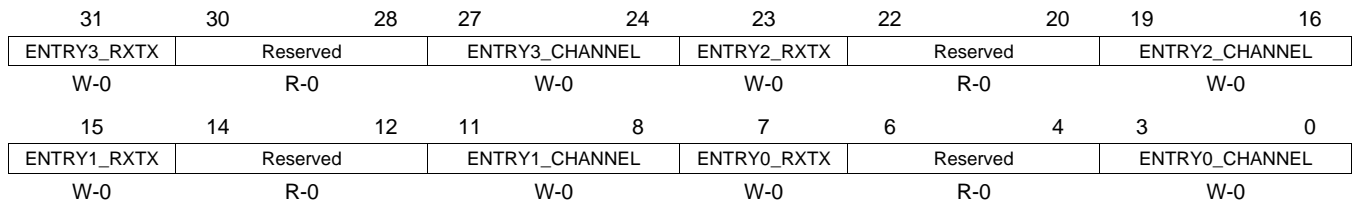
Figure 100. CDMA Scheduler Table Word n Registers (WORD[n])
