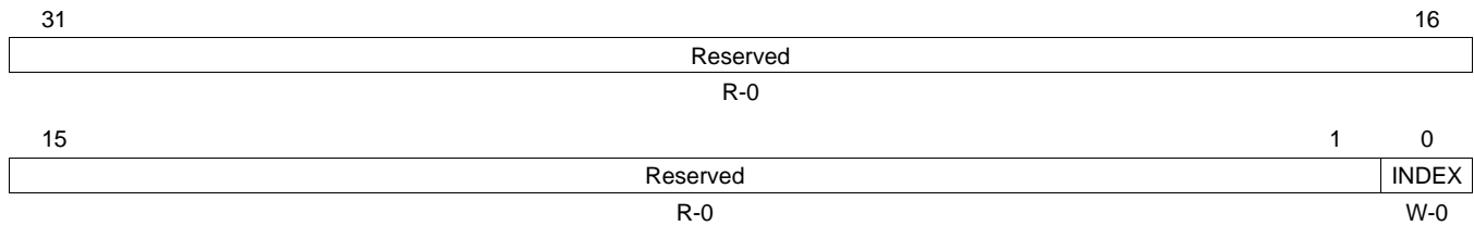
Figure 11-11. Host Interrupt Enable Indexed Set Register (HEISR)
