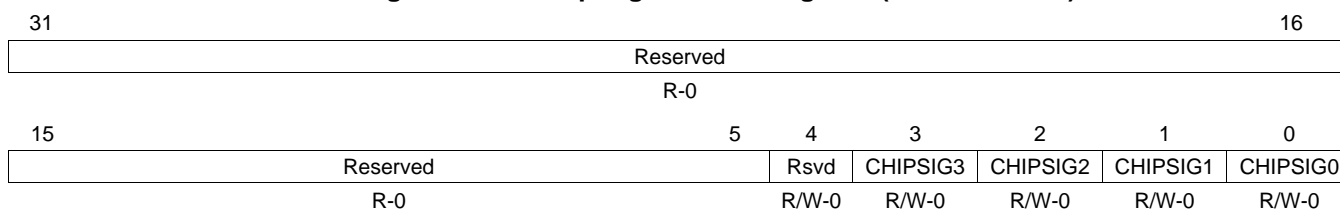
Figure 10-39. Chip Signal Clear Register (CHIPSIG_CLR)
