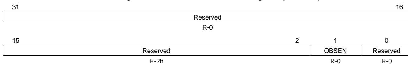
Figure 7-34. PLLC1 Clock Status Register (CKSTAT)
