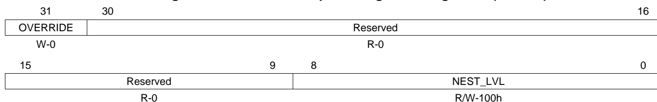
Figure 11-38. Host Interrupt Nesting Level Register 2 (HINLR2)
