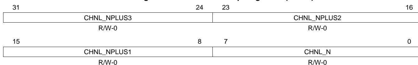
Figure 11-34. Channel Map Registers (CMRn)
