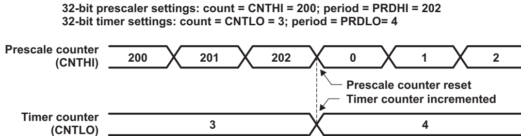
Figure 2-3 Dual 32-Bit Timers Chained Mode Example
