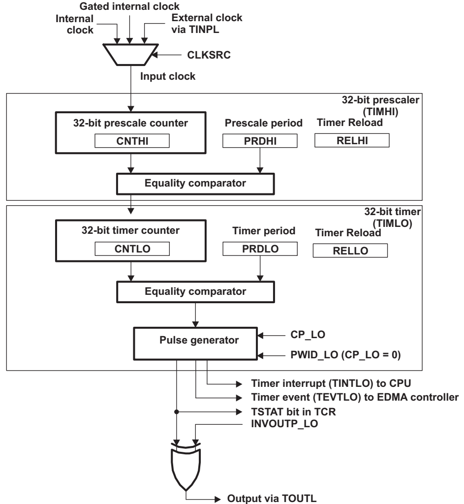
Figure 2-2 Dual 32-Bit Timers Chained Mode Block Diagram
