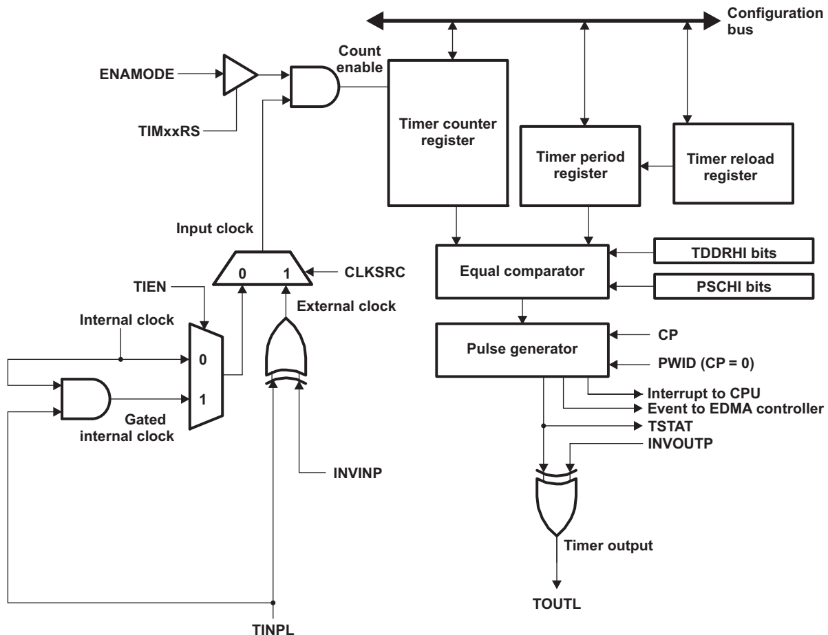
Figure 1-1 Timer Block Diagram
