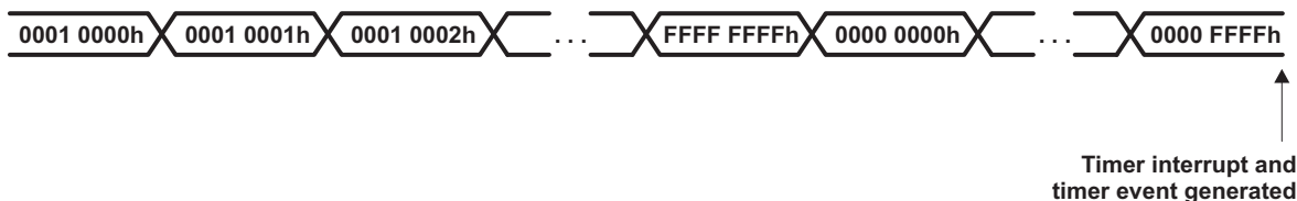
Figure 3-2 32-Bit Timer Counter Overflow Example
