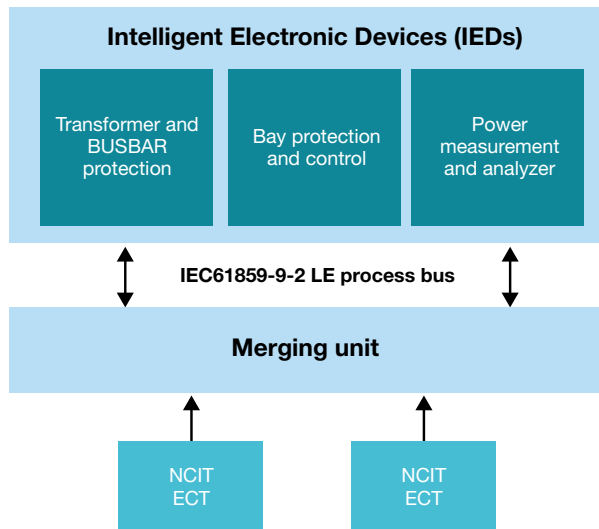
Figure 5. A merging unit interfaced to non-conventional instrument transformers.
