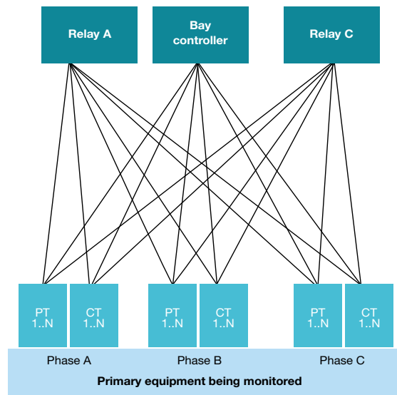
Figure 1. CT and PT wiring in a conventional substation using copper wires.
