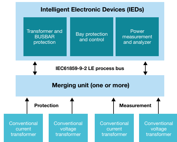
Figure 3. A merging unit with a conventional transformer
