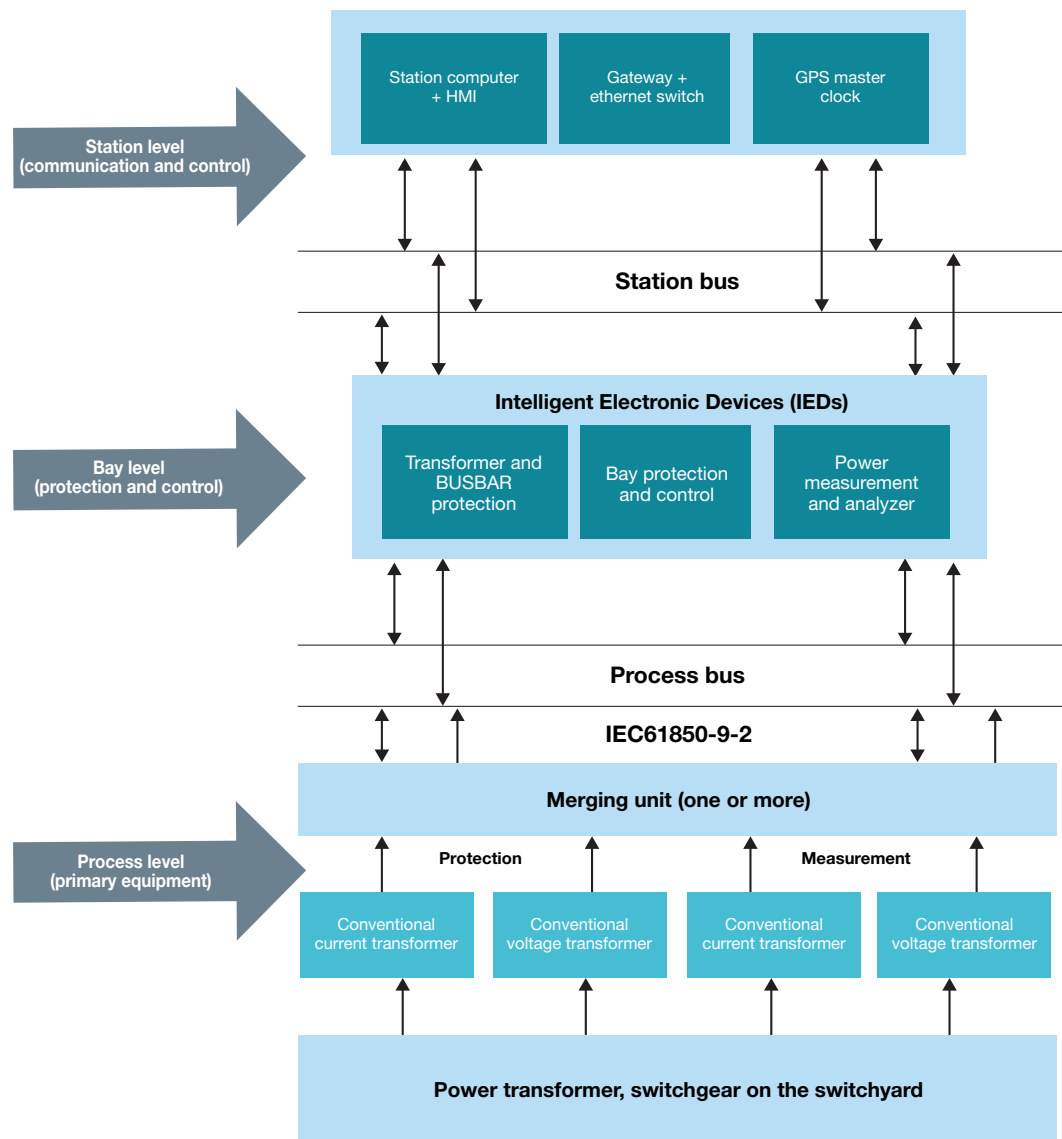
Figure 2. Digital substation architecture.
