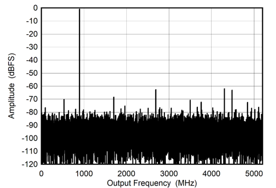
Figure 5-6. DES Mode: Single Tone FFT at 897 MHz
