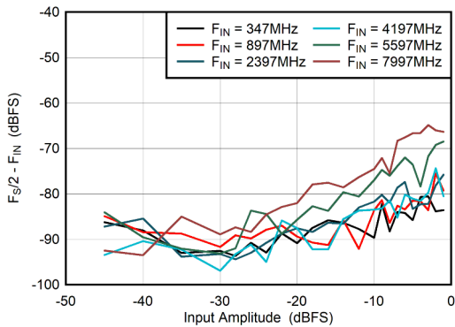
Figure 5-79. Dual Channel Mode: F_S/2 - F_{IN} vs Input Amplitude
