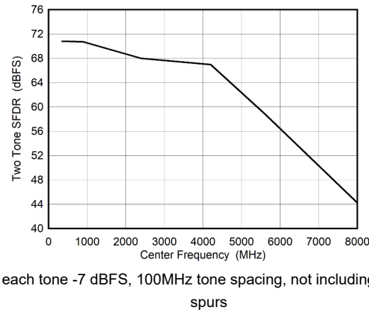
Figure 5-108. Dual Channel Mode: Two Tone SFDR vs Input Frequency
