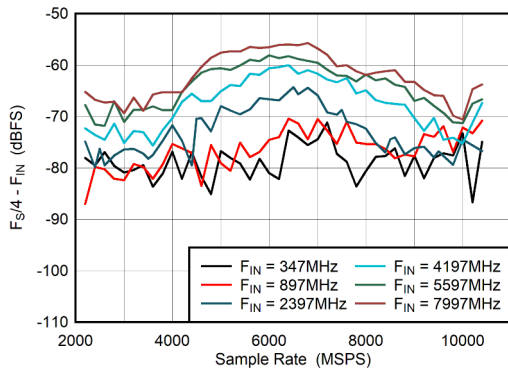
Figure 5-43. DES Mode: F_S/4 - F_{IN} vs Sample Rate
