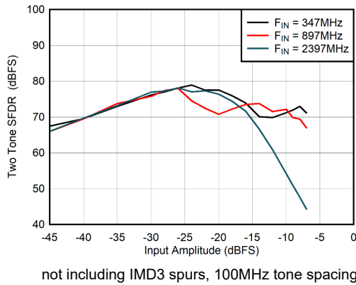
Figure 5-109. Dual Channel Mode: Two Tone SFDR vs Input Amplitude
