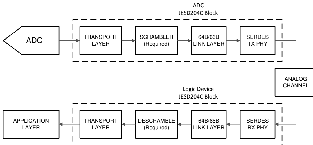
Figure 6-9. Simplified 64B/66B Encoded JESD204C Interface Diagram
