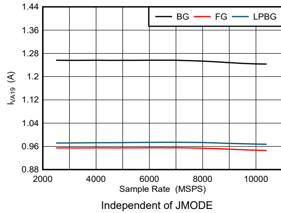
Figure 5-110. DES Mode: I_{VA19} vs Sample Rate
