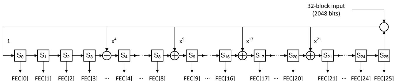
Figure 6-11. FEC Parity Bit Generator
