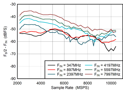
Figure 5-41. DES Mode: F_S/2 - F_{IN} vs Sample Rate
