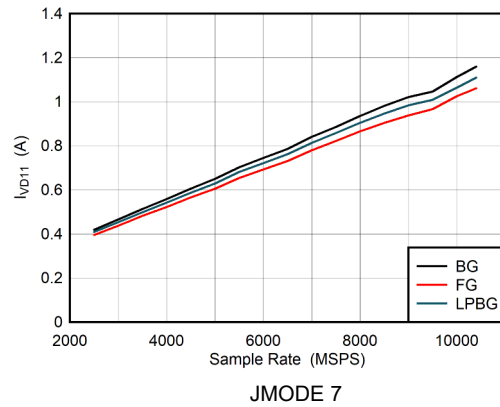
Figure 5-112. DES Mode: I_{VD11} vs Sample Rate
