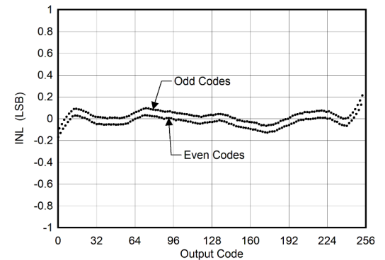
Figure 5-4. INL vs ADC Code
