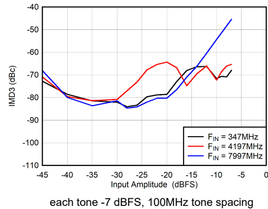
Figure 5-106. Dual Channel Mode: IMD3 vs Input Amplitude
