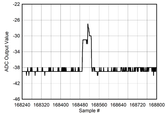
Figure 5-120. Background Calibration Core Transition (AC Signal Zoomed)
