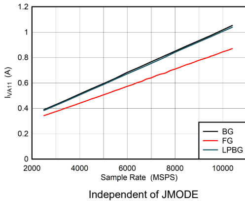
Figure 5-111. DES Mode: I_{VA11} vs Sample Rate
