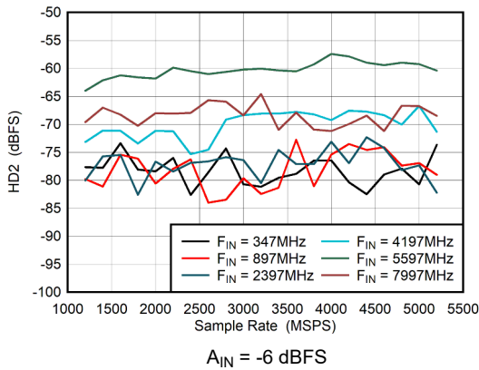
Figure 5-51. Dual Channel Mode: HD2 vs Sample Rate
