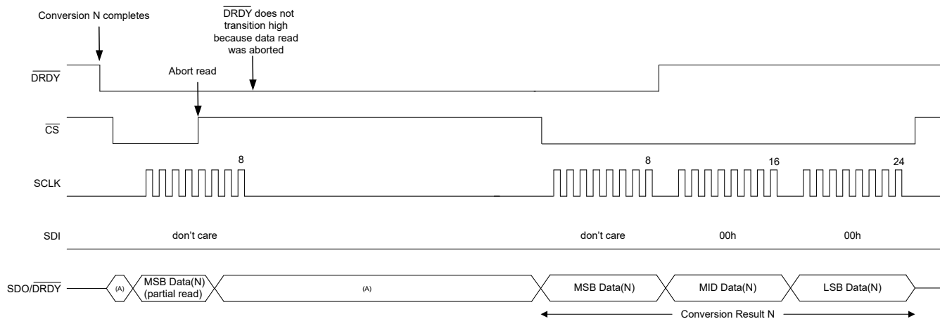
Figure 7-63. \overline{\text{DRDY}} Pin Behavior: Incomplete Read of Conversion Data Before New Conversions Complete
