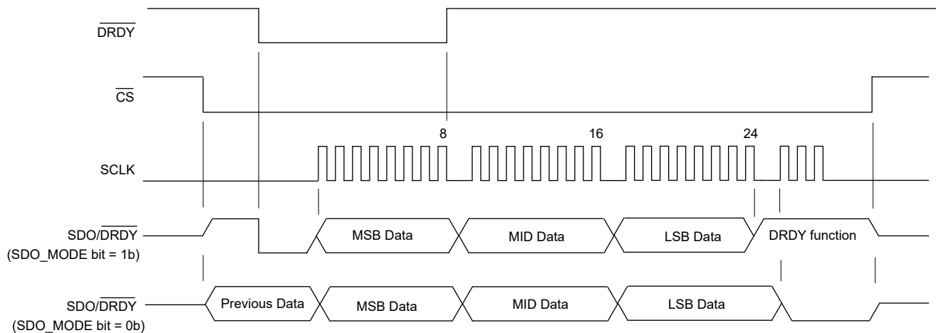
Figure 7-42. SDO/ \overline{\text{DRDY}} and \overline{\text{DRDY}} Function With Additional SCLK Pulses
