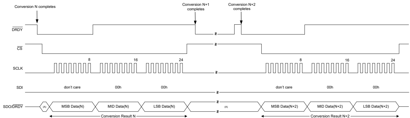
Figure 7-65. DRDY Pin Behavior: Reading Conversion Data While New Conversions Complete
