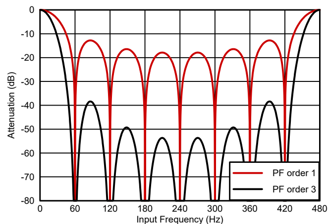
Figure 7-33. Parallel Post Filter Frequency Response, 8 averages and scan rate of 480Hz
