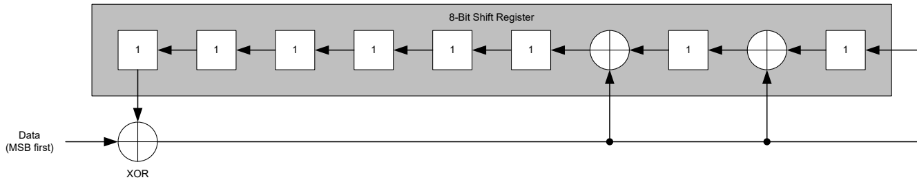
Figure 7-44. Visual Representation of CRC Calculation
