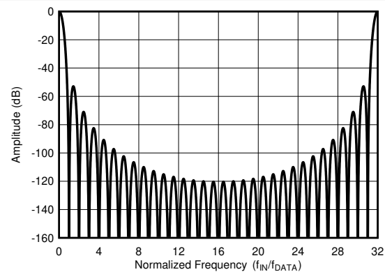
Figure 7-13. Sinc4 Frequency Response to f_{\text{MOD}} (OSR = 32)
