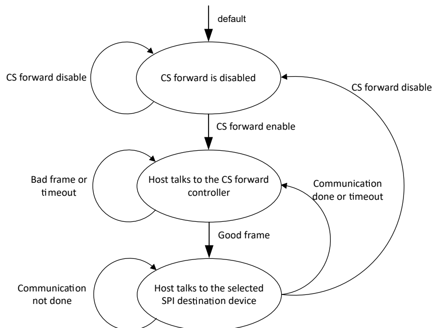
Figure 7-38. CS Forward State Diagram
