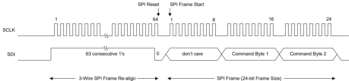
Figure 7-74. 3-Wire Mode SPI Re-Align Pattern
