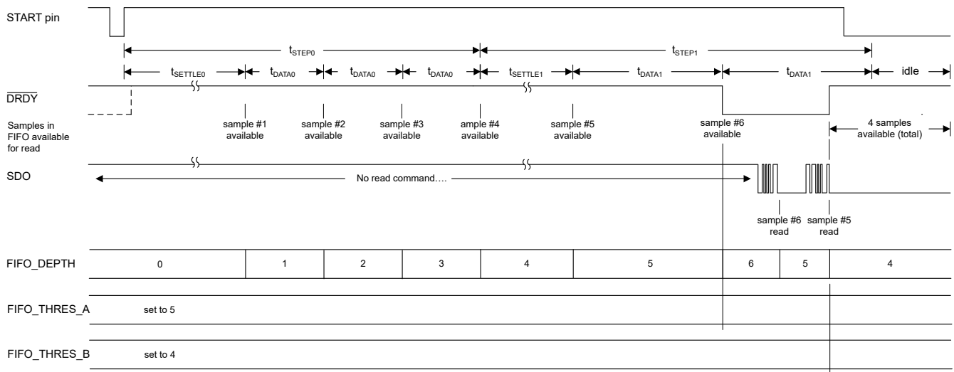
Figure 7-26. \overline{\text{DRDY}} Behavior Based on FIFO Thresholds
