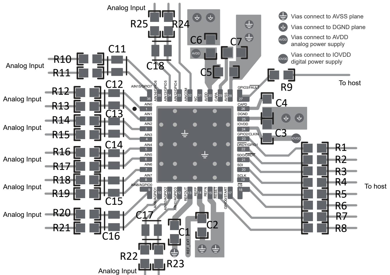
Figure 8-10. Layout Example
