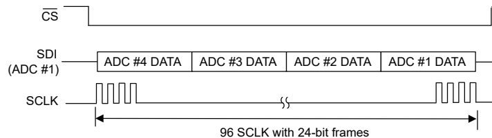
Figure 7-70. 24 bit Data Input Sequence
