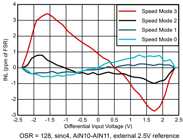
Figure 5-6. INL vs Differential Input Voltage
