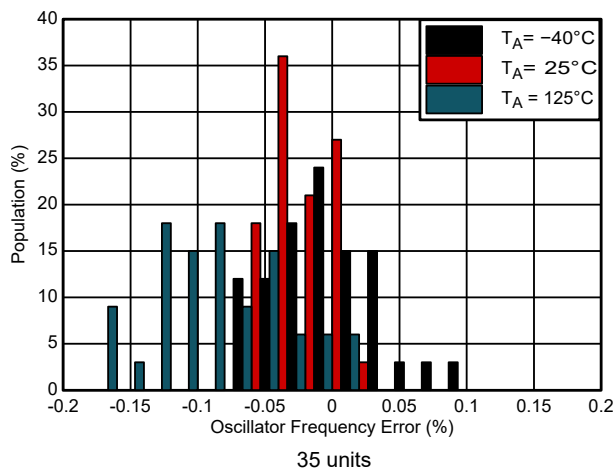
Figure 5-10. Internal Oscillator Frequency Histogram
