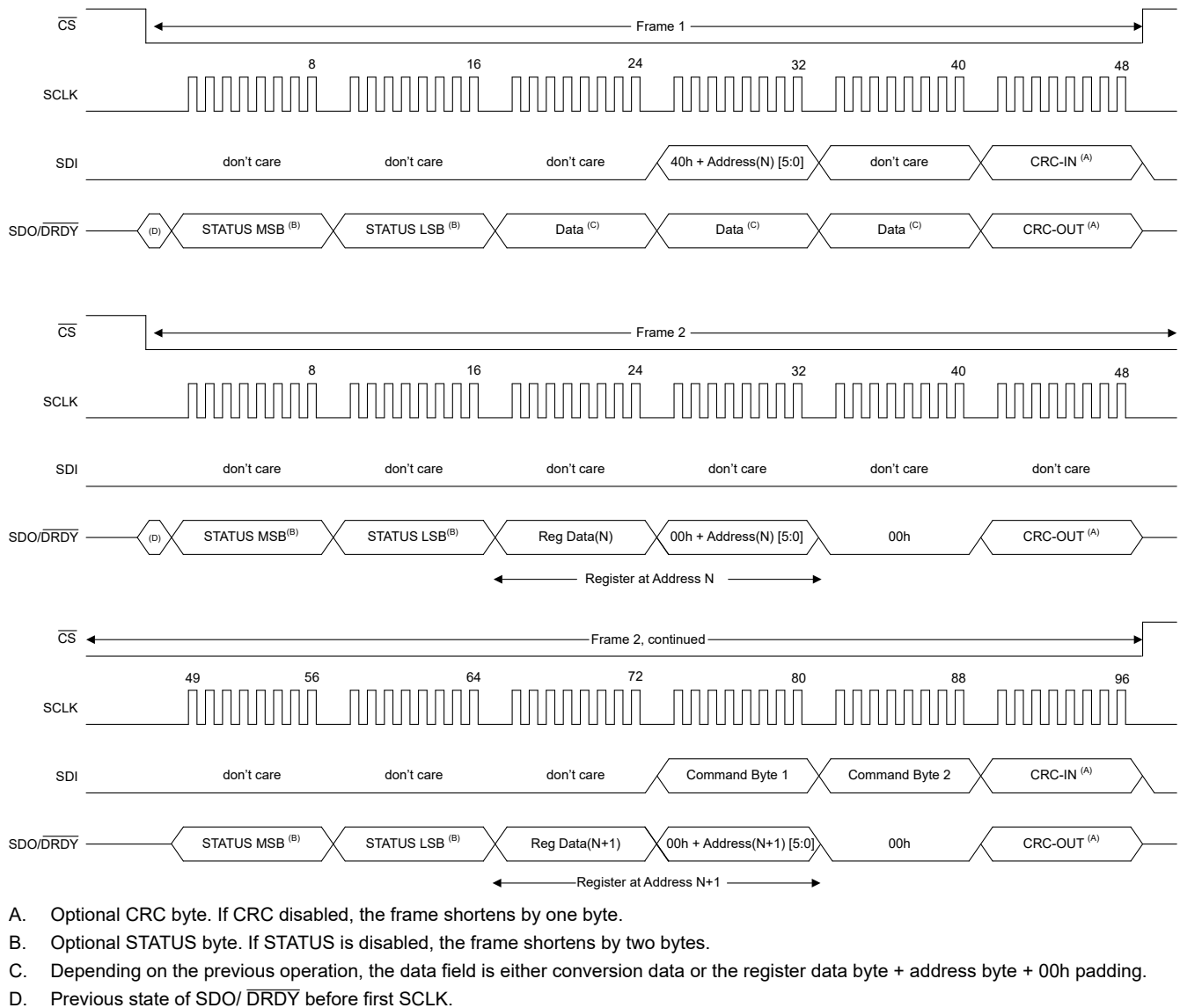
Figure 7-58. Read Register Data in Continuous Read Mode, STATUS Header and CRC Byte Enabled
