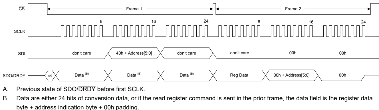
Figure 7-47. Read Register Data, 24-Bit Frame Size
