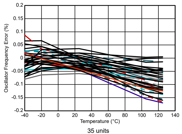
Figure 5-11. Internal Oscillator Frequency vs Temperature
