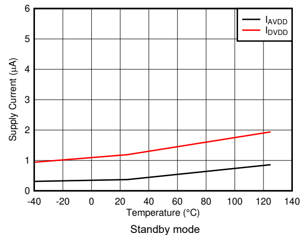
Standby mode Figure 6-15. Supply Current vs Temperature
