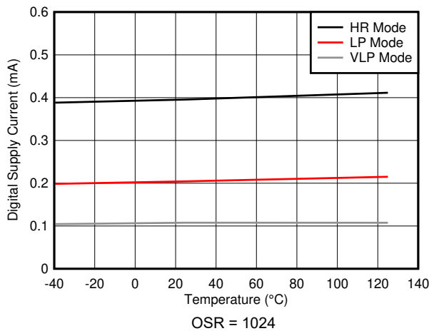
OSR = 1024 Figure 6-14. Digital Supply Current vs Temperature
