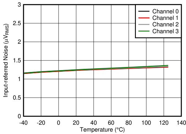
Gain = 8, global-chop mode disabled Figure 6-10. Input-referred Noise vs Temperature
