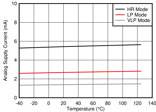
Gain = 1, OSR = 1024, all four ADC channels enabled Figure 6-12. Analog Supply Current vs Temperature
