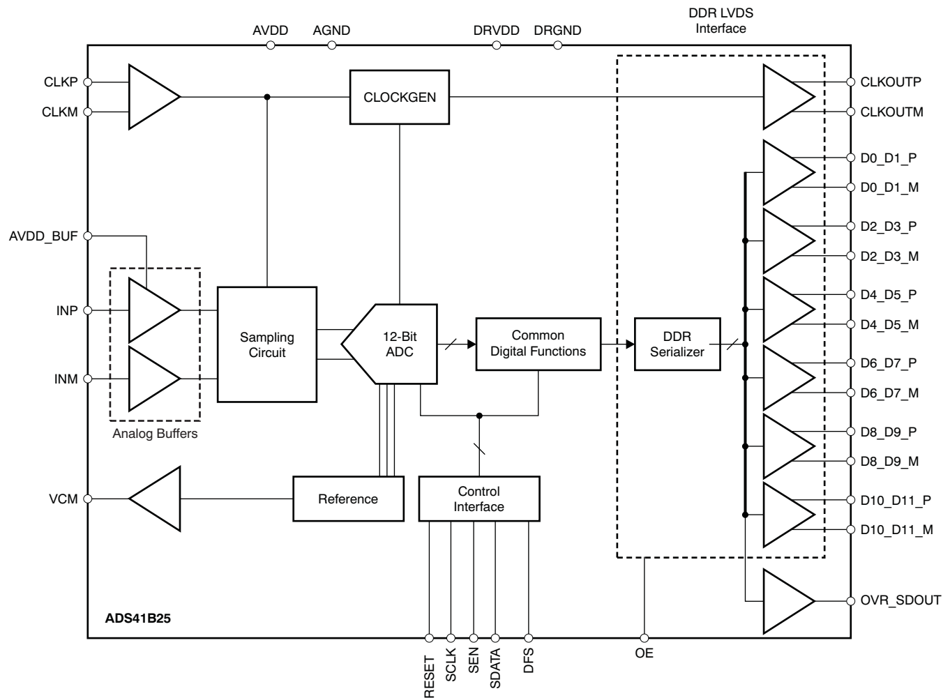
Figure 3. Block Diagram
