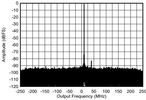
Figure 4-430. RX Single Tone Output FFT at 8.1 GHz, -1 dBFS
