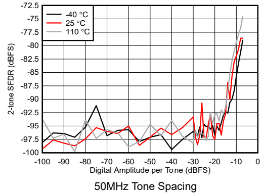
Figure 4-429. RX 2-tone SFDR vs Digital Amplitude at 8.1 GHz
