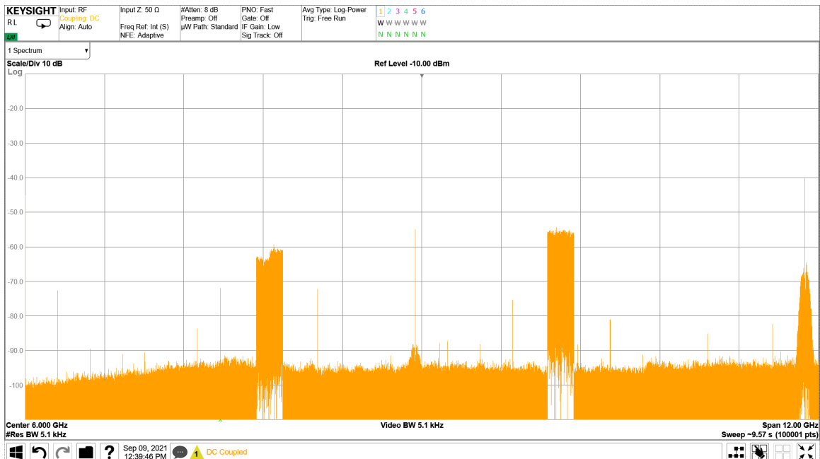
Figure 4-226. TX 4x100 MHz NR Output Spectrum 8.1 GHz
