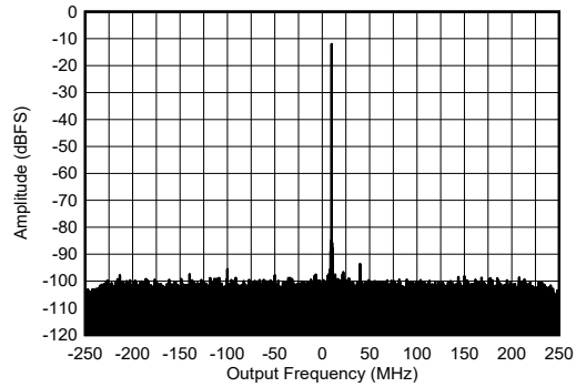
Figure 4-431. RX Single Tone Output FFT at 8.1 GHz, -3 dBFS
