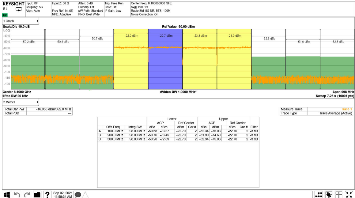
Figure 4-225. TX 4x100 MHz NR Output Spectrum 8.1 GHz
