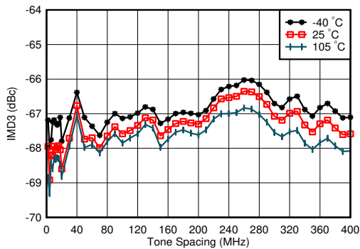
f_{DAC} = 11796.48 MSPS, interleaved mode, matching at 4.9 GHz, f_{CENTER} = 4.9 GHz, -13 dBFS each tone, worst channel
