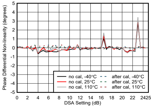
Figure 4-416. RX Phase Differential Nonlinearity at 8.11 GHz
