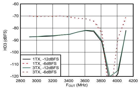
Matching at 3.5 GHz, f_{DAC} = 11.79648 GSPS, interleave mode, normalized to output power at harmonic frequency. Dip is due to HD3 falling near DC.
