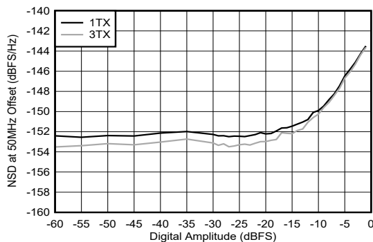
50 MHz offset
