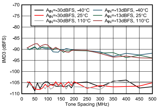
Figure 4-420. RX IMD3 vs Tone Spacing at 8.11 GHz
