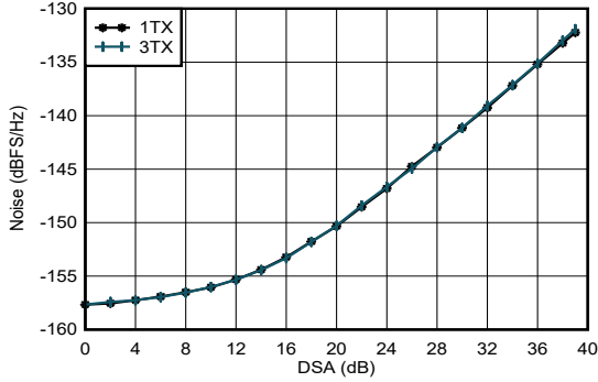
A. f_{DAC} = 11796.48 MSPS, interleave mode, matching at 3.5 GHz, A_{out} = -13 dBFS.
