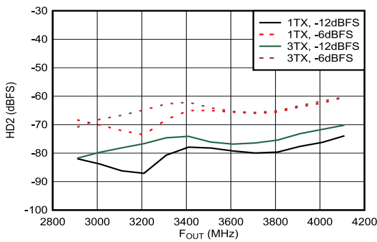
Matching at 3.5 GHz, f_{DAC} = 11.79648 GSPS, interleave mode, normalized to output power at harmonic frequency
