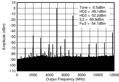
Figure 4-179. TX Single Tone (-12 dBFS) Output Spectrum at 4.9 GHz ( 0-f_{DAC} )
