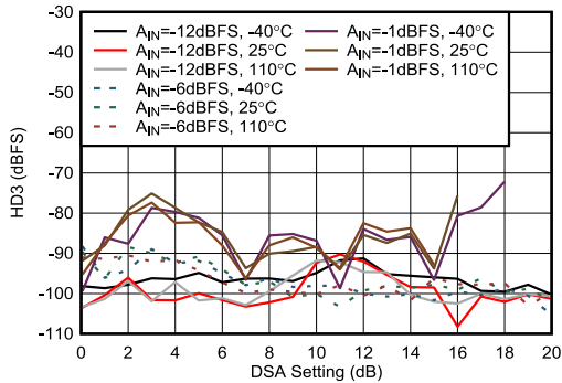
Figure 4-428. RX HD3 vs DSA Setting at 8.1 GHz
