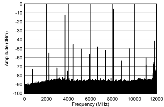
Figure 4-201. TX Single Tone Output Spectrum at 8.1 GHz
