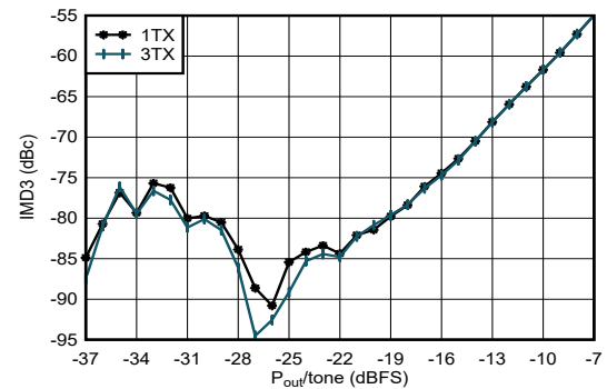
f_{DAC} = 11796.48 MSPS, interleaved mode, matching at 4.9 GHz, f_{CENTER} = 4.9 GHz, f_{SPACING} = 20 MHz
