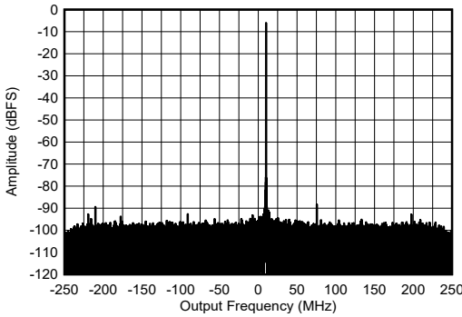
Figure 4-430. RX Single Tone Output FFT at 8.1 GHz, -1 dBFS
