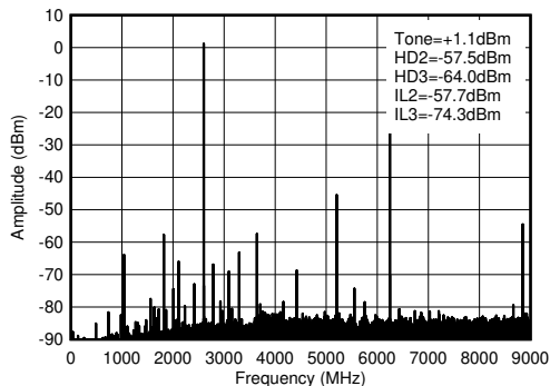
Figure 4-112. TX Single Tone (-12 dBFS) Output Spectrum at 2.6 GHz ( 0-f_{DAC} )
