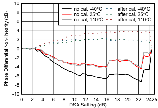
Figure 4-417. RX Phase Differential Nonlinearity at 8.11 GHz
