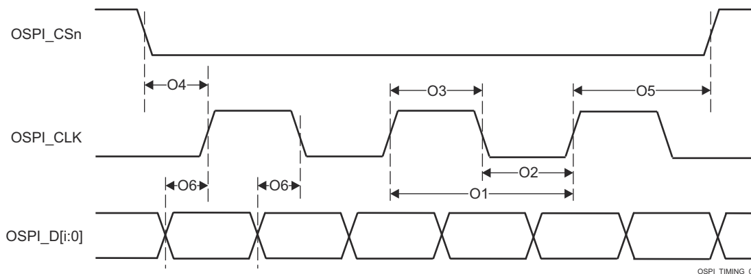
Figure 6-104. OSPI0 Switching Characteristics – PHY DDR
