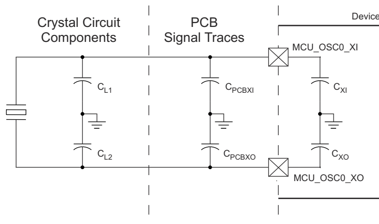
Figure 6-18. Load Capacitance
