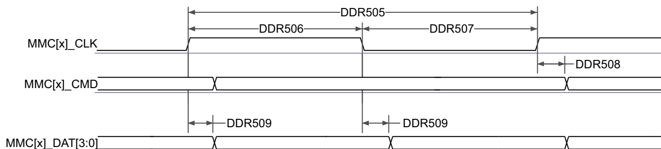
Figure 6-83. MMC0 – UHS-I DDR50 – Transmit Mode
