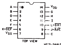
CD4023B
