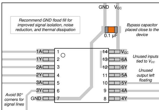
Figure 7-1. Layout Diagram
