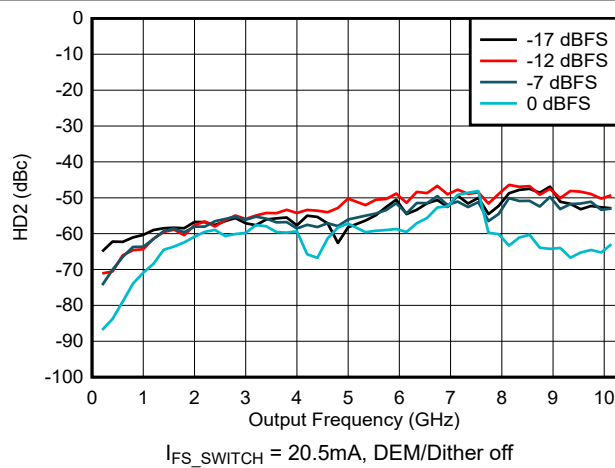
Figure 6-160. HD2 vs Frequency and Digital Amplitude in NRZ/RF Modes
