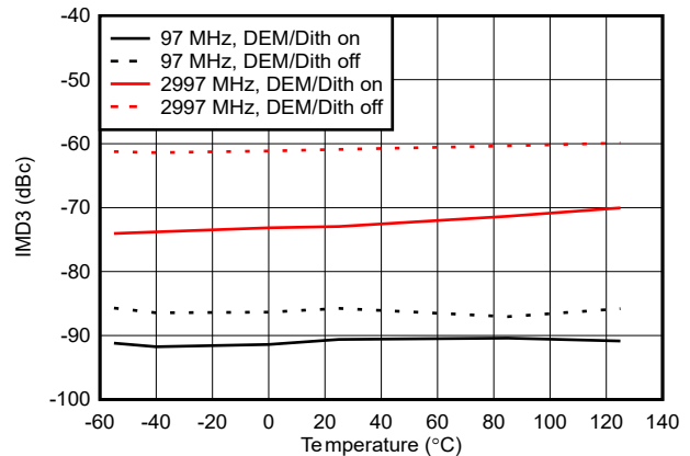
Figure 6-149. IMD3 vs Temperature in DES2XL Mode
