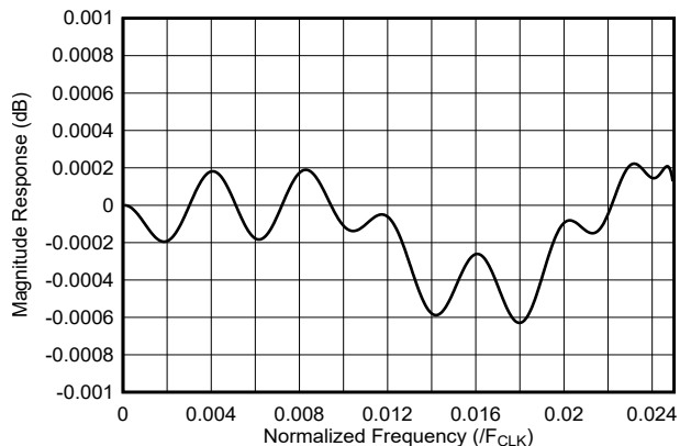
Figure 7-27. 16x Interpolation Filter Passband Response
