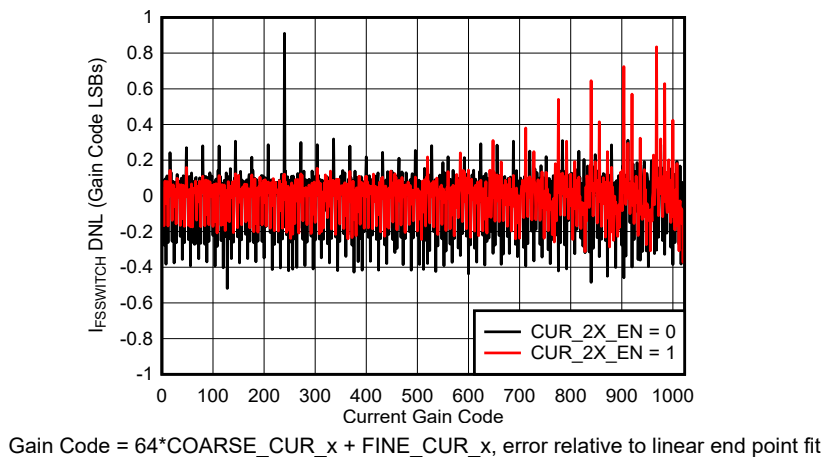
Figure 6-18. I_{\text{FS\_SWITCH}} Error Differential Non-Linearity vs Gain Code
