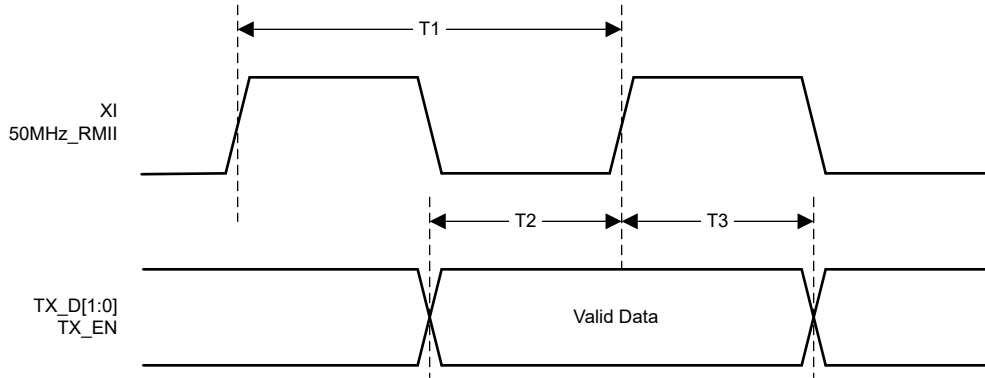
Figure 7-4. RMIITransmit Timing
