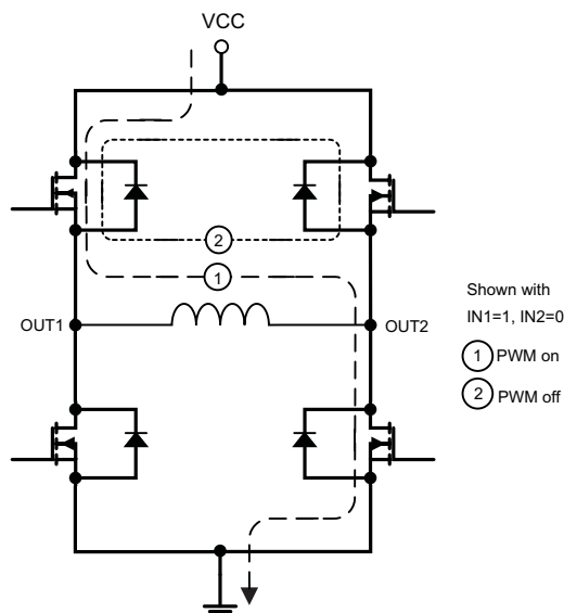
Figure 8. Voltage Regulation
