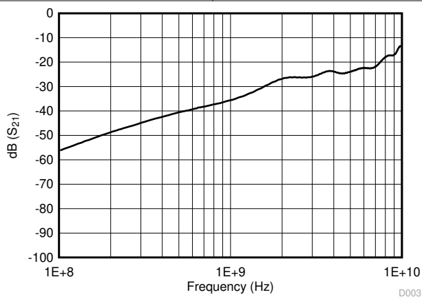
Figure 6-3. Off Isolation
