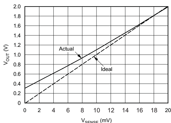
Figure 38. Example for Low V_{SENSE} Cases 1 and 3 (INA208, Gain = 100)
