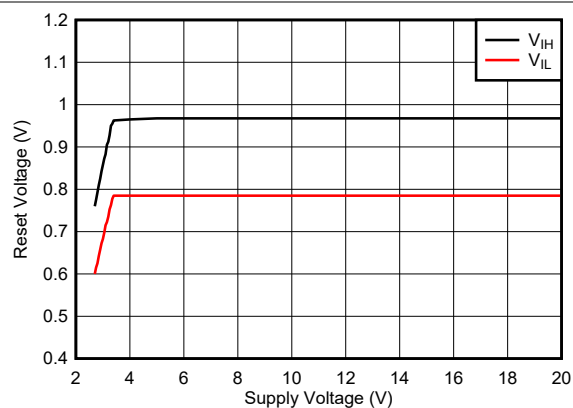
Figure 6-38. Comparator Reset Voltage vs Supply Voltage
