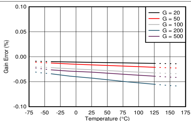
Figure 6-10. INA310A-Q1 Gain Error vs Temperature
