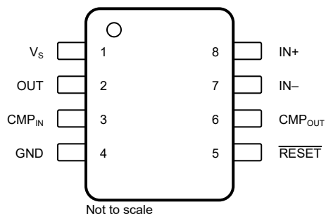
Figure 5-1. INA310x-Q1: DKG Package 8-Pin VSSOP Top View
