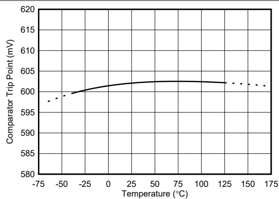
Figure 6-36. Comparator Trip Point vs Temperature
