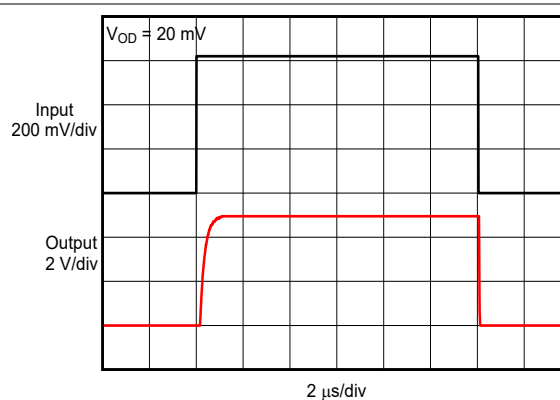
Figure 6-40. Comparator Propagation Delay
