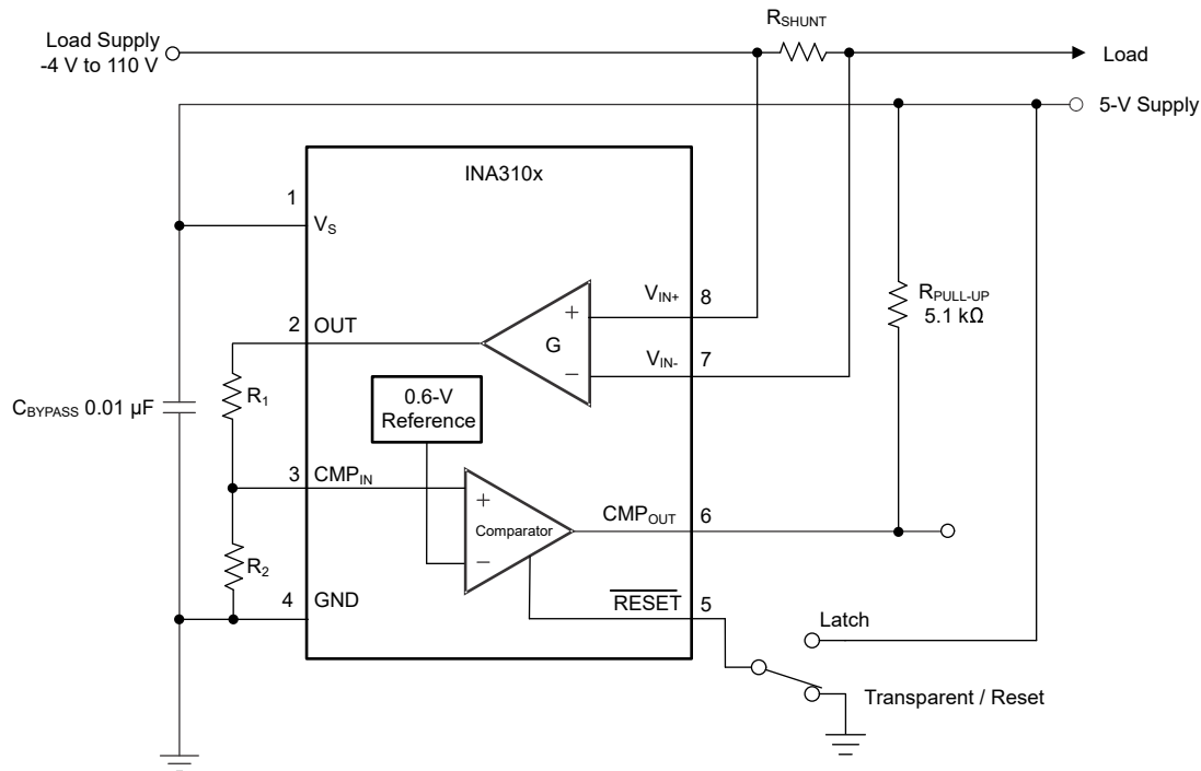
Figure 7-4. INA310x-Q1 Basic Connections
