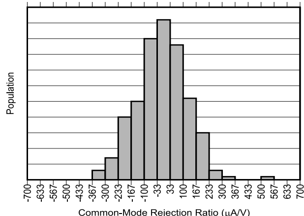
Figure 5-6. INA751B Common-Mode Rejection Production Distribution
