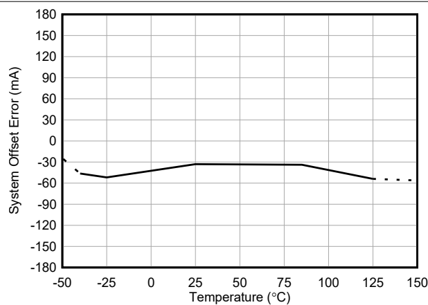
Figure 5-4. INA751B Input Offset Current vs Temperature
