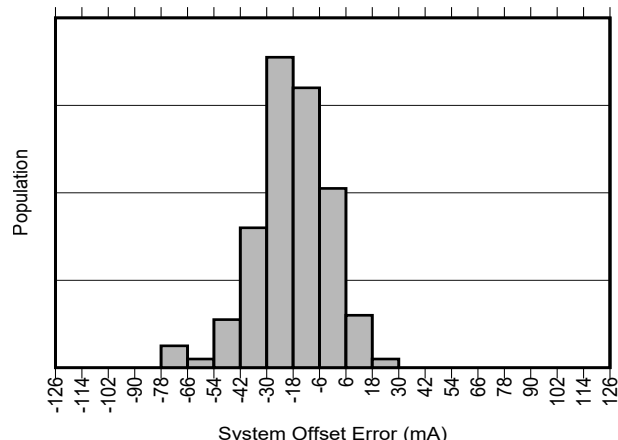
Figure 5-2. INA751B Input Offset Current Production Distribution
