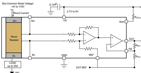
Typical Application
