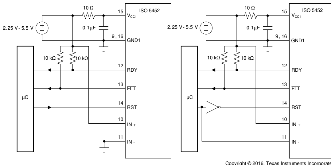
Figure 10-7. Auto Reset for Noninverting and Inverting Input Configuration
