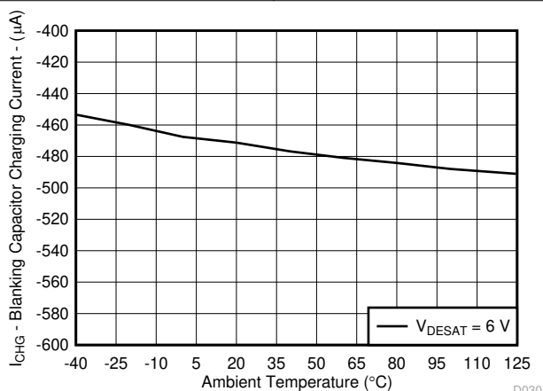
V_{CC2} = 15 \text{ V} DESAT = 6 \text{ V} Figure 7-43. Blanking Capacitor Charging Current vs Temperature
