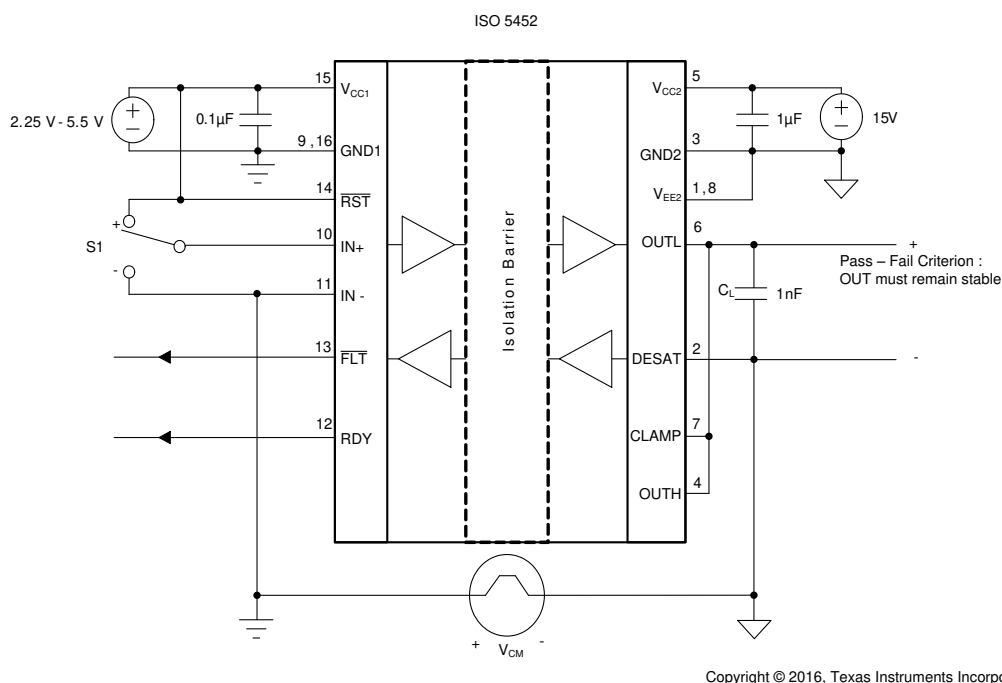
Figure 8-4. Common-Mode Transient Immunity Test Circuit
