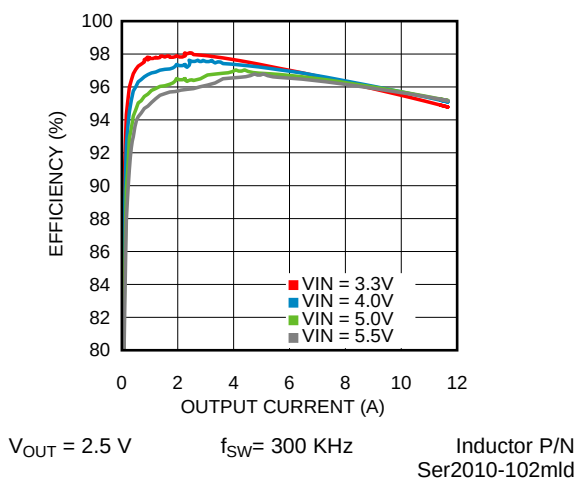
Figure 3. Efficiency
