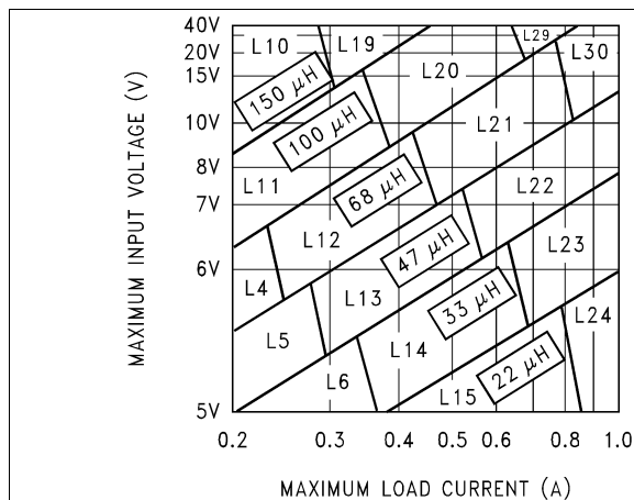
Figure 27. LM2595 3.3-V
