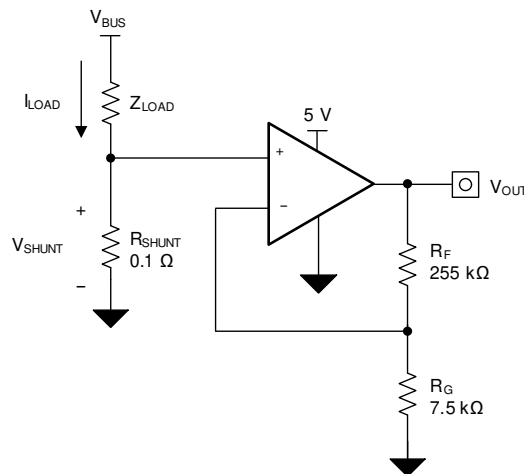
Figure 8-1. LM290xLV Device in a Low-Side, Current-Sensing Application
