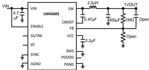
V_{OUT} = 1\text{ V} F_S = 500\text{ kHz}
