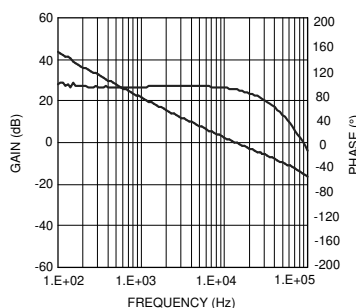
Figure 8-6. Overall Loop Gain and Phase
