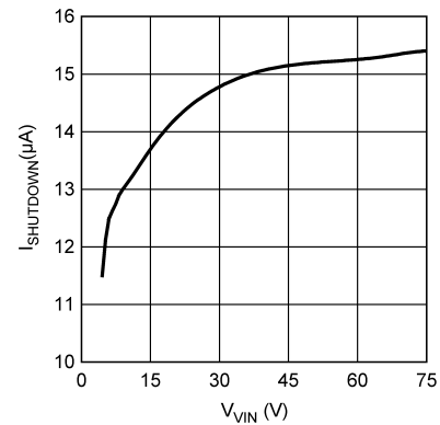
Figure 6-4. Shutdown Current
