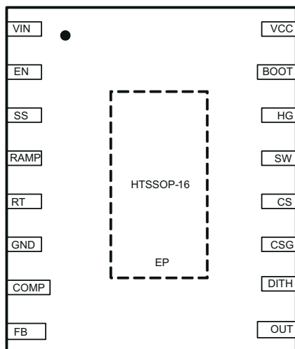
Figure 5-1. 16-Pin PWP Package (Dither Version) (Top View)
