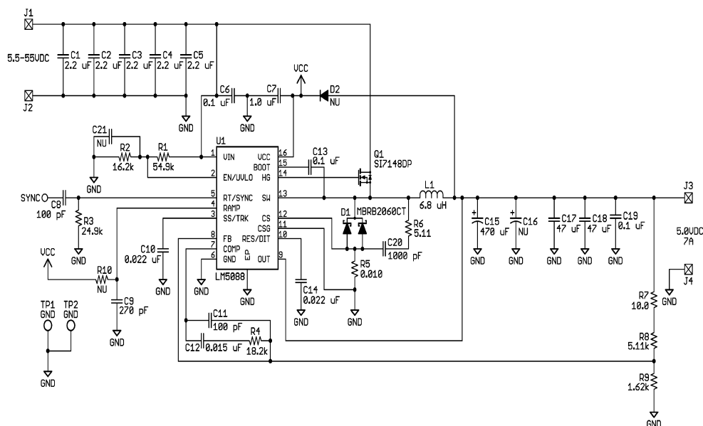
Figure 9-2. LM5088-2 Application Schematic
