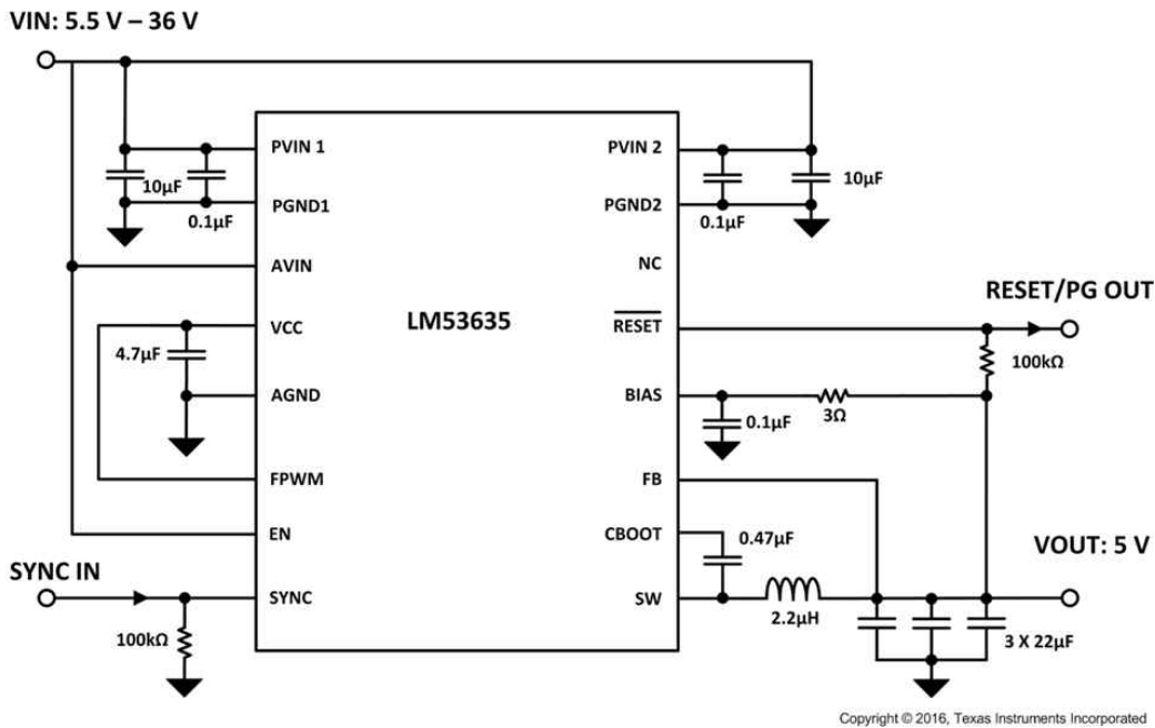
Figure 9-4. Fixed 5-V, 3.5-A Output Power Supply
