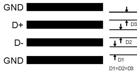
Figure 16. Ideal Diode Trace Layout
