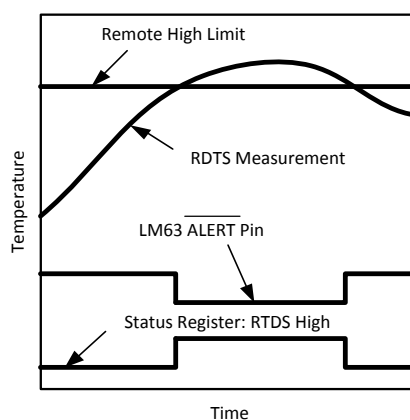
Figure 7. \overline{\text{ALERT}} Output as Temperature Comparator Response Diagram
