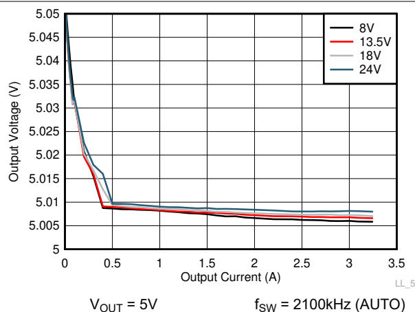
Figure 8-12. Line and Load Regulation
