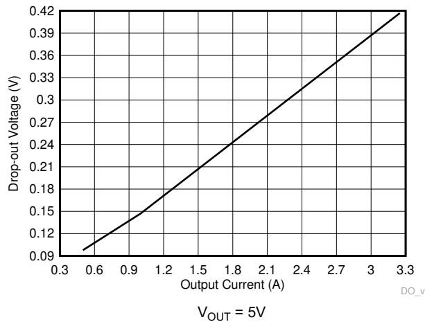
Figure 8-16. Dropout Voltage versus Output Current for -1% Drop
