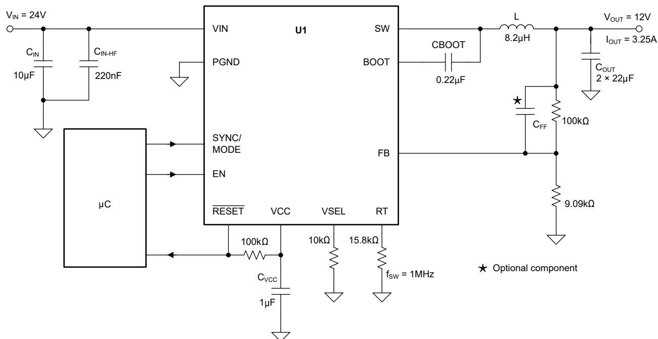
Figure 8-7. Full-Featured Design Example V_{IN} = 24V , V_{OUT} = 12V , I_{OUT} = 3.25A , f_{SW} = 1MHz
