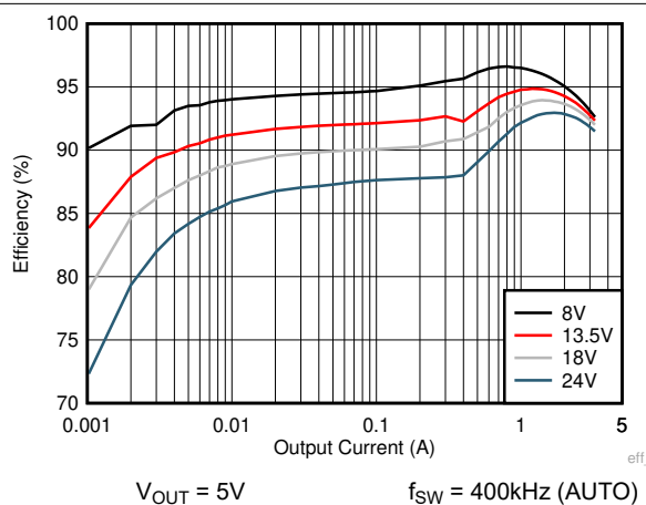
Figure 8-10. Efficiency
