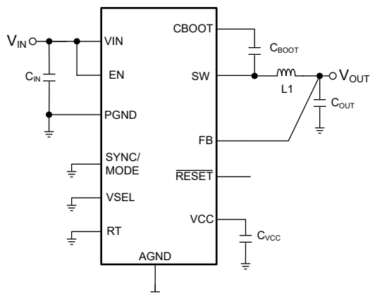
Simplified Schematic
