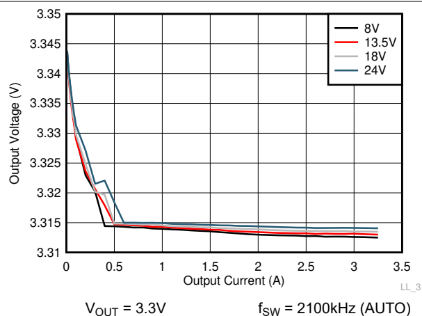
Figure 8-13. Line and Load Regulation
