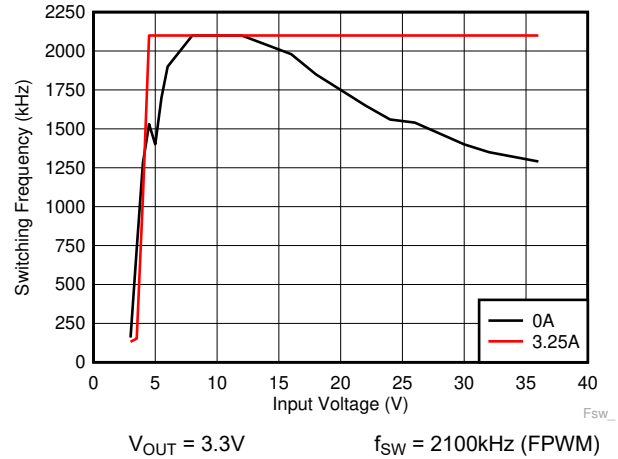
Figure 8-15. Switching Frequency versus Input Voltage
