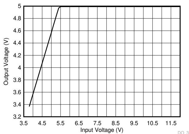
Figure 7-11. Overall Dropout Characteristic V_{OUT} = 5V , I_{OUT} = 3.25A
