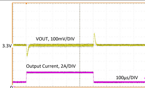
Figure 8-23. Load Transient
