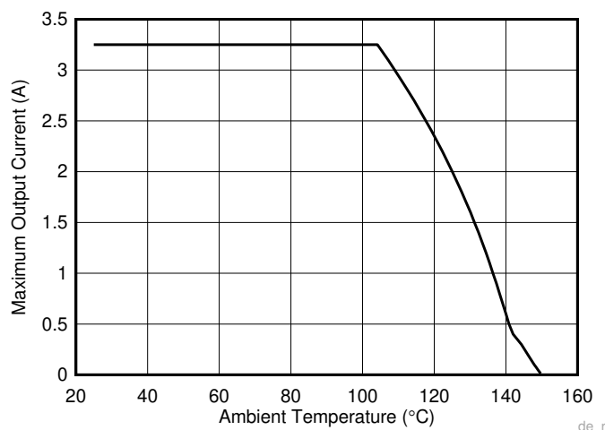
Figure 8-6. Maximum Output Current versus Ambient Temperature V_{IN} = 12V , V_{OUT} = 5V , f_{SW} = 400kHz , R_{\theta JA} = 22^{\circ}C/W
