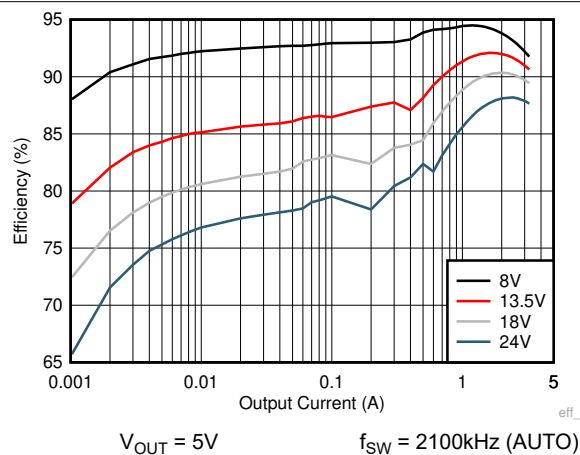
Figure 8-8. Efficiency
