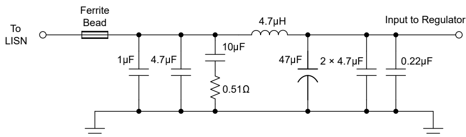
A. Input filter used only for EMI measurements shown in EMI Performance Curves .
