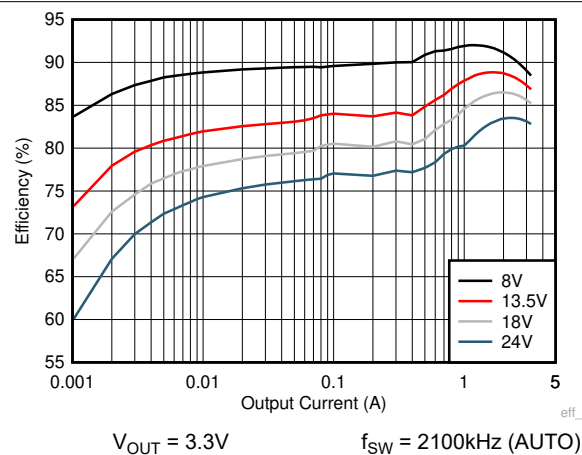
Figure 8-9. Efficiency
