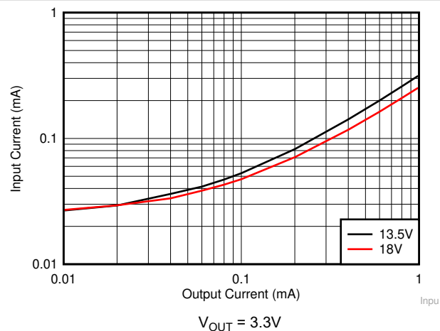
Figure 8-19. Input Supply Current versus Output Current
