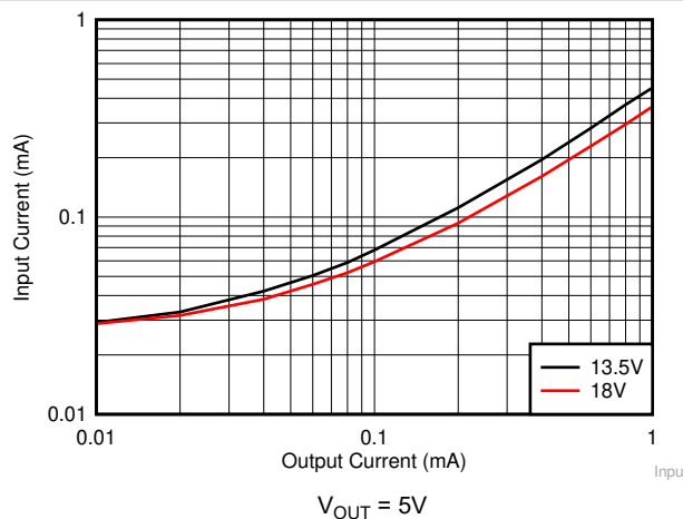
Figure 8-18. Input Supply Current versus Output Current
