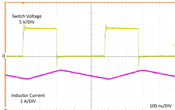
Figure 7-7. Typical PWM Switching Waveforms Without Spread Spectrum V_{IN} = 12V , V_{OUT} = 5V , I_{OUT} = 3.25A , f_{SW} = 2100kHz
