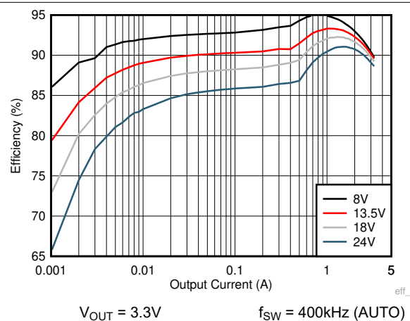
Figure 8-11. Efficiency
