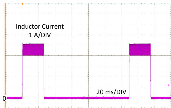
Figure 7-12. Inductor Current Burst in Short-Circuit Mode
