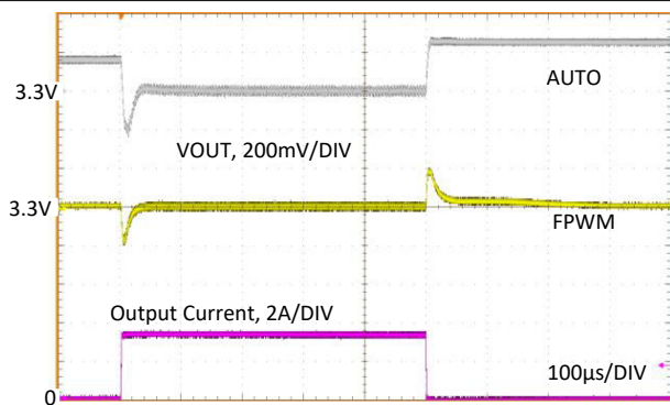
Figure 8-21. Load Transient
