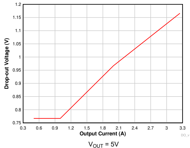
Figure 8-17. Dropout Voltage versus Output Current to 1.85MHz
