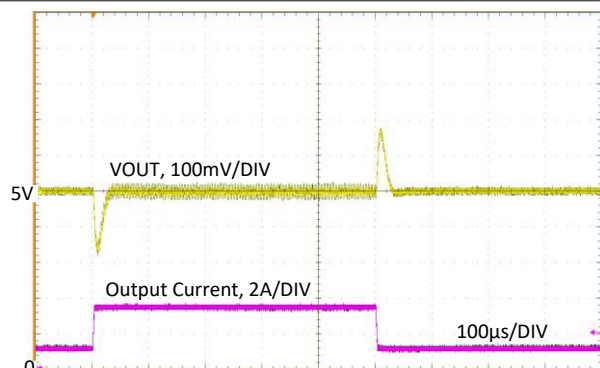
Figure 8-22. Load Transient
