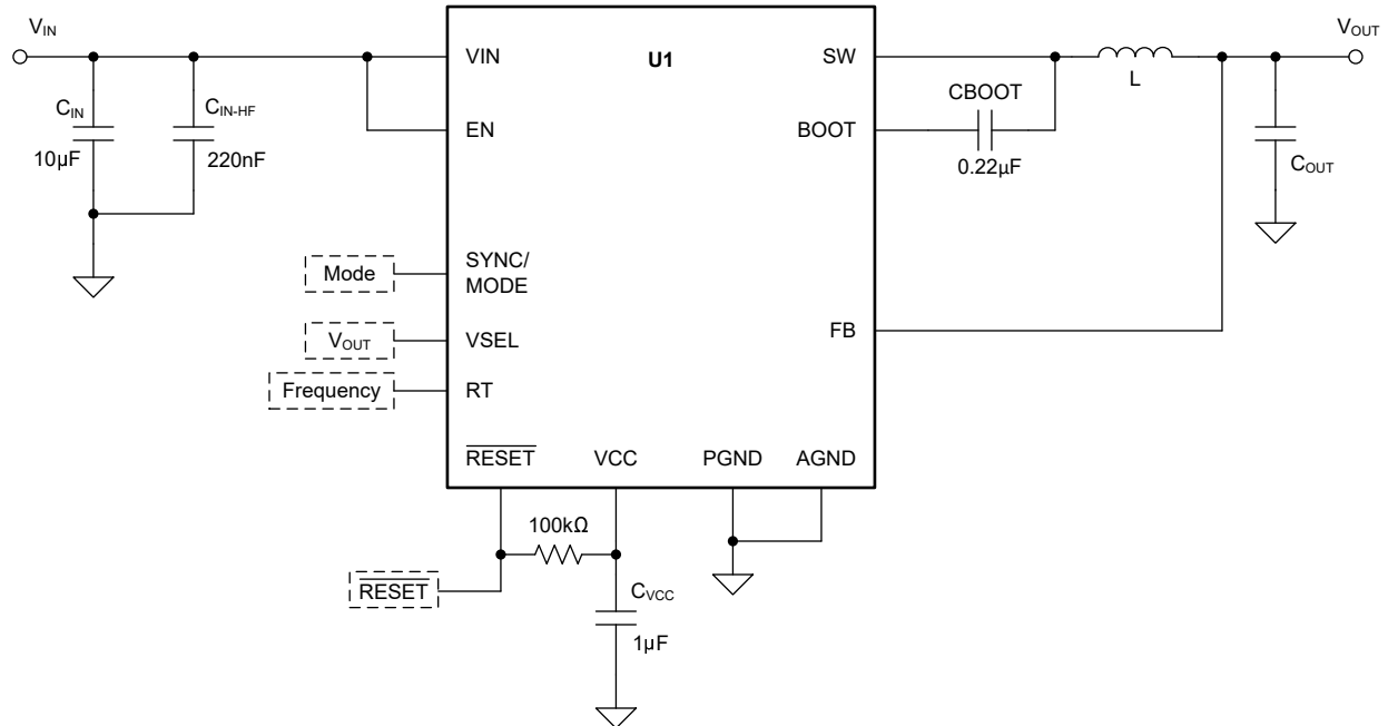
Figure 8-26. Circuit for Typical Application Curves
