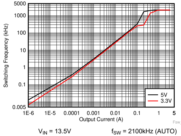
Figure 8-14. Switching Frequency versus Output Current
