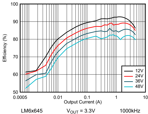
Figure 8-39. LM6x645 Efficiency - Auto Mode
