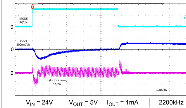
Figure 8-91. MODE Change Transient
