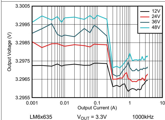
Figure 8-47. LM6x635 Line and Load Regulation - Auto Mode
