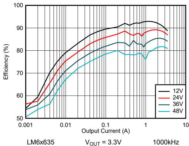
Figure 8-35. LM6x635 Efficiency - Auto Mode
