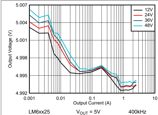
Figure 8-19. LM6xx25 Line and Load Regulation - Auto Mode
