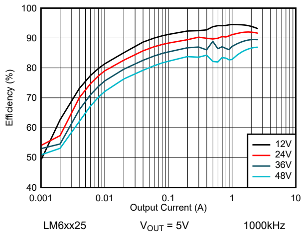
Figure 8-33. LM6xx25 Efficiency - Auto Mode
