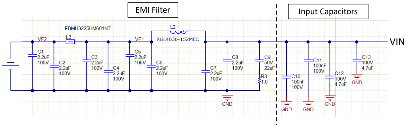
Figure 8-95. EMI Input Filter for 2200kHz
