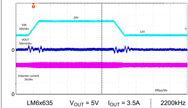
Figure 8-93. Line Transient - Auto
