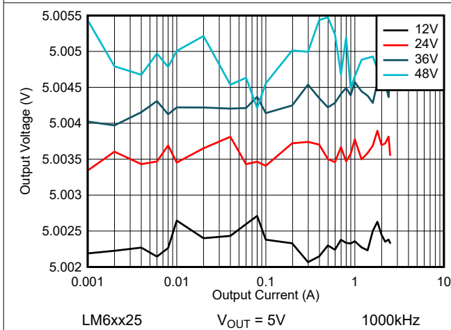
Figure 8-45. LM6xx25 Line and Load Regulation - Auto Mode
