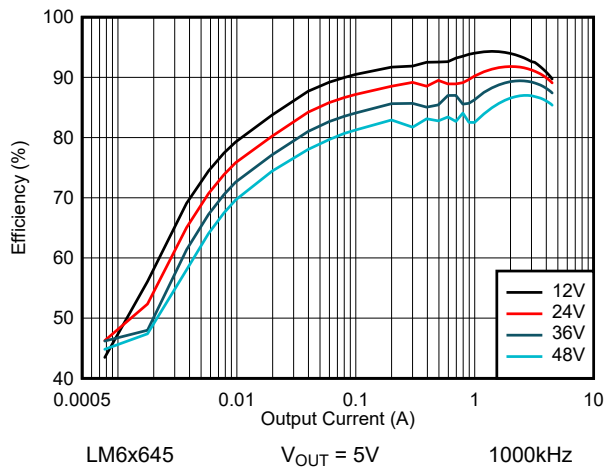
Figure 8-41. LM6x645 Efficiency - Auto Mode
