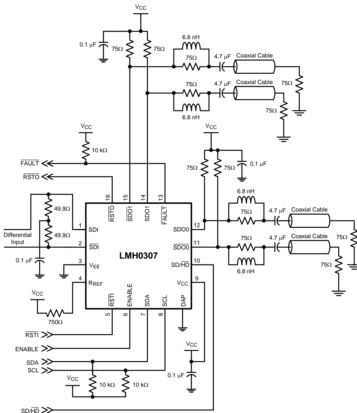
Figure 4. Application Circuit
