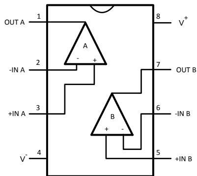
8-Pin SOIC and VSSOP (LMH6643) Package DKG08A Top View
