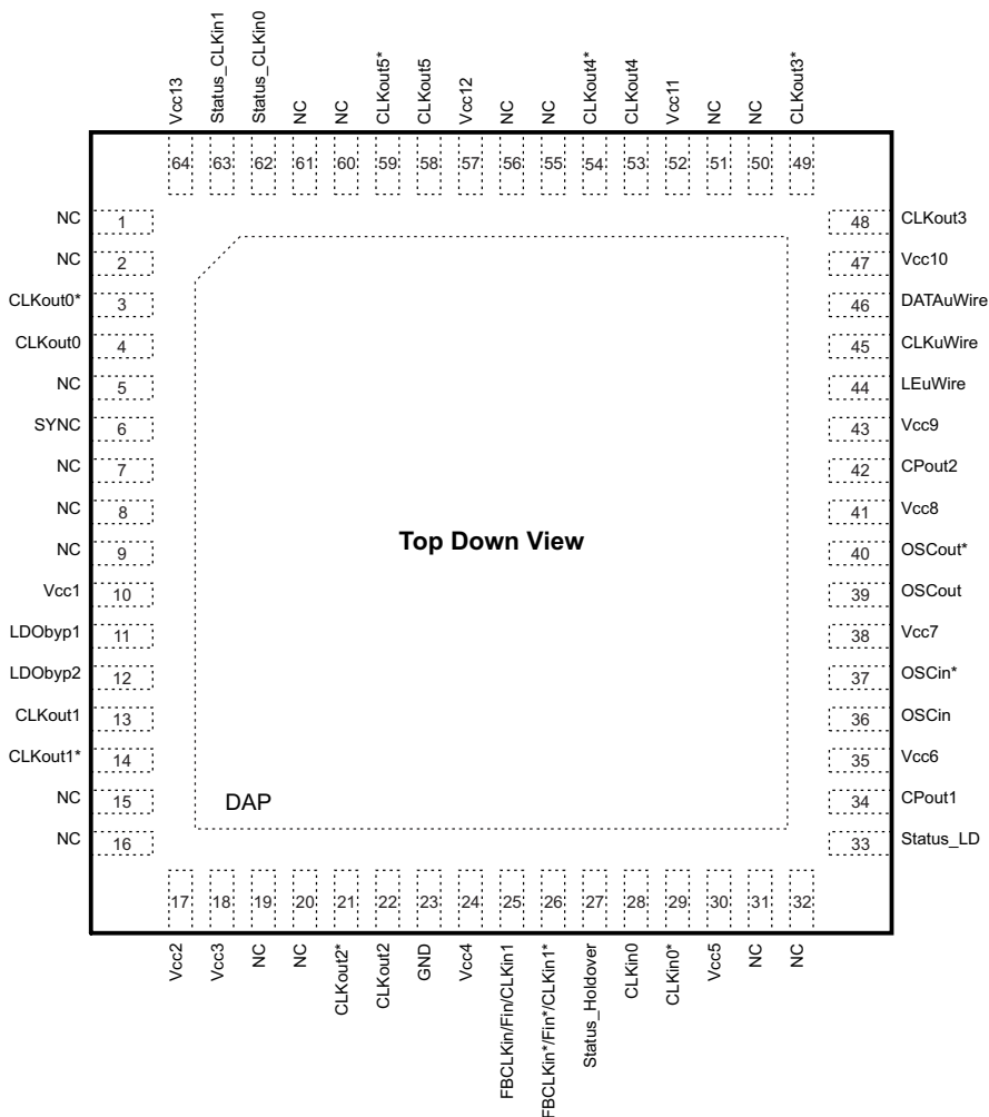
Pin Functions (1)
