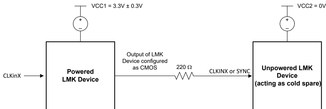
Figure 9-7. Cold Sparing Devices Setup
