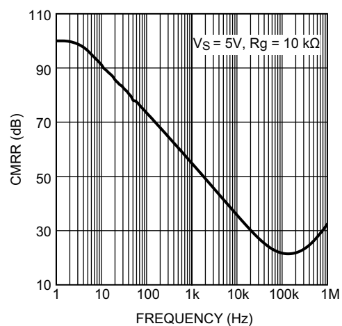
Figure 6-4. AC CMRR vs. Frequency
