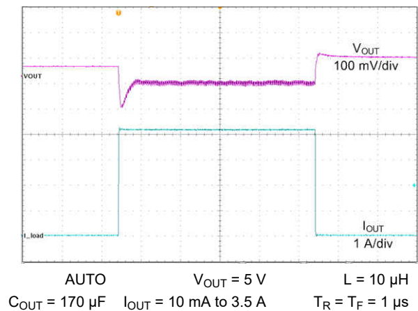
Figure 9-14. Load Transients
