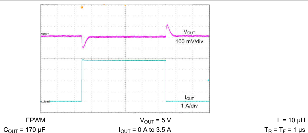
Figure 9-15. Load Transient
