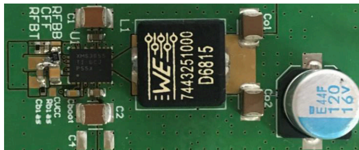
Figure 11-3. LMS3655MQEVM Layout
