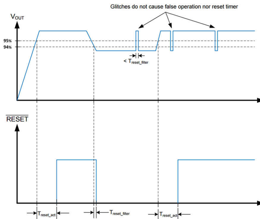
Figure 8-3. \overline{\text{RESET}} Timing Behavior
