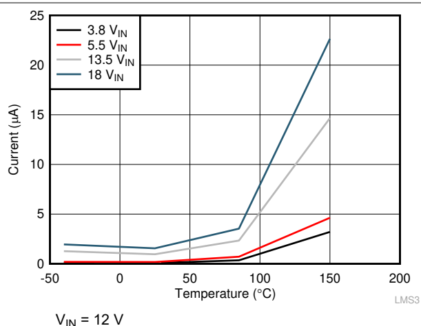
Figure 7-6. Shutdown Current
