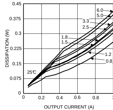
Figure 8. Dissipation 8-V Input at 25°C
