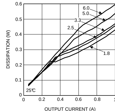
Figure 10. Dissipation 12-V Input at 25°C
