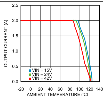
Figure 48. Thermal Derating V_{OUT} = 12 \text{ V} , R_{\theta JA} = 16^\circ\text{C/W}
