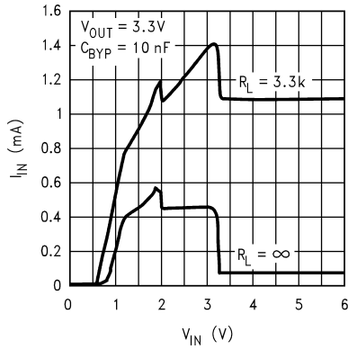
Figure 5-31. Input Current vs Input Voltage (Legacy Chip)
