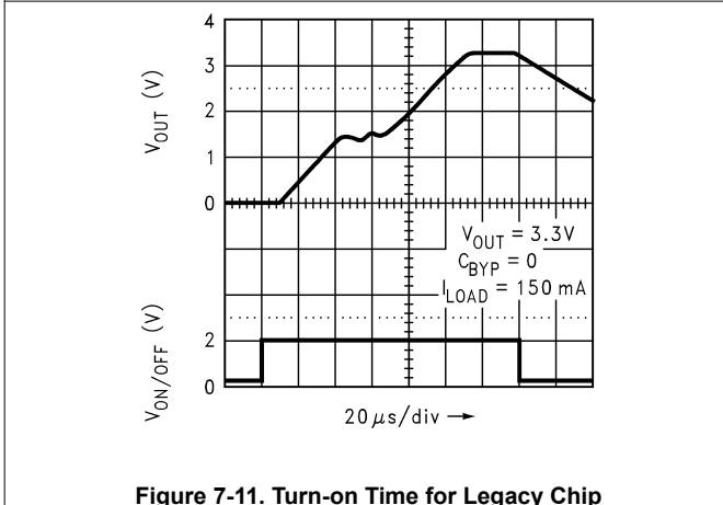
Figure 7-11. Turn-on Time for Legacy Chip
