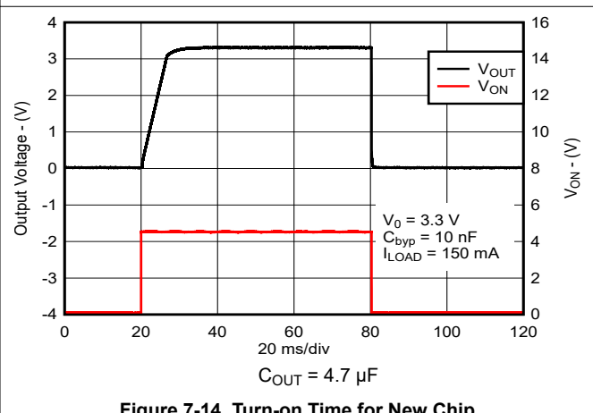
Figure 7-14. Turn-on Time for New Chip
