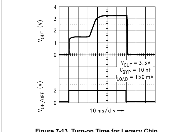
Figure 7-13. Turn-on Time for Legacy Chip
