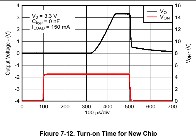
Figure 7-12. Turn-on Time for New Chip
