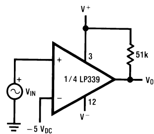
Comparator With a Negative Reference
