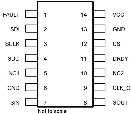
Figure 5-1. LP5899 DYY Package 14-pin SOT-23-THN Top View
